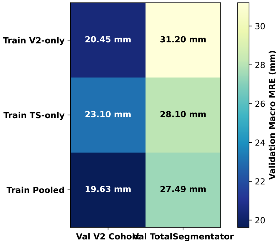
Cross-Domain Transfer Matrix (65-Epoch Matched)
