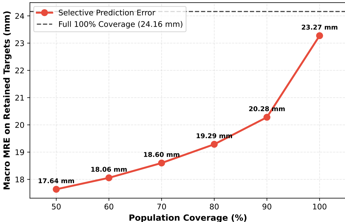
Uncertainty Risk-Coverage Curve (Ensemble Disagreement)
