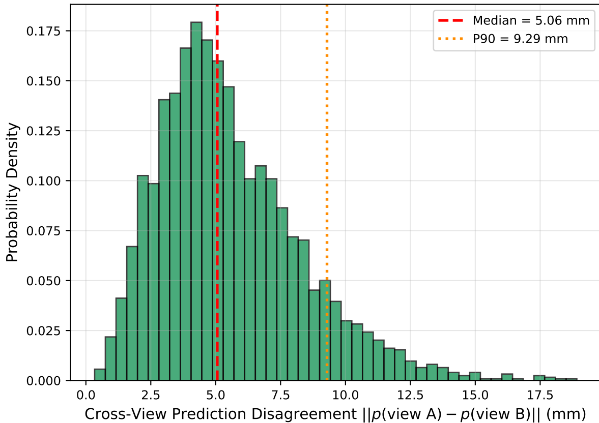
Figure 11: HuMMan Cross-View Mutual Prediction Consistency
