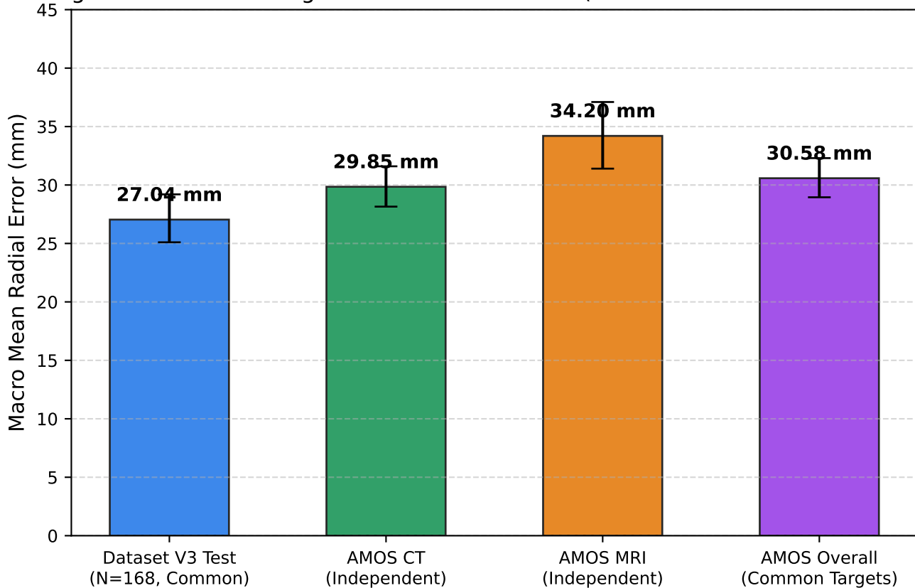
Figure 4: Common-Target Internal Localization (Dataset V3 vs AMOS External)
