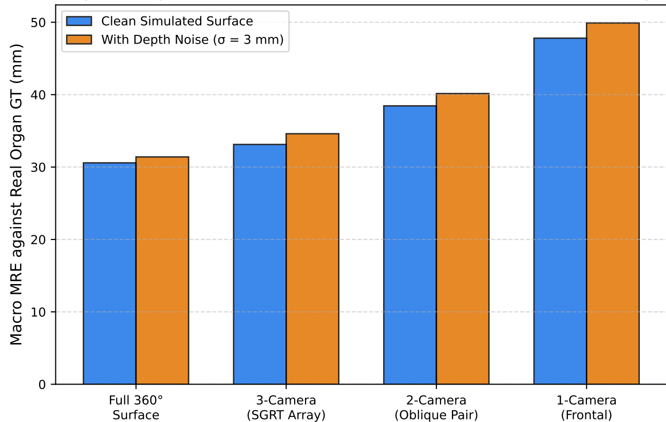
Figure 7: Optical Camera Simulation on AMOS External Torso Geometry
