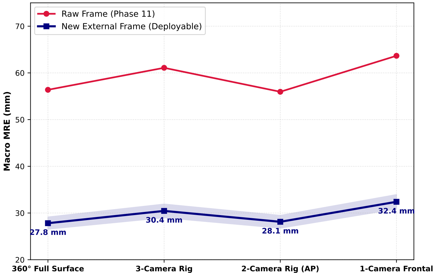
FIGURE 10: Optical Camera Robustness After Canonical Frame Correction
