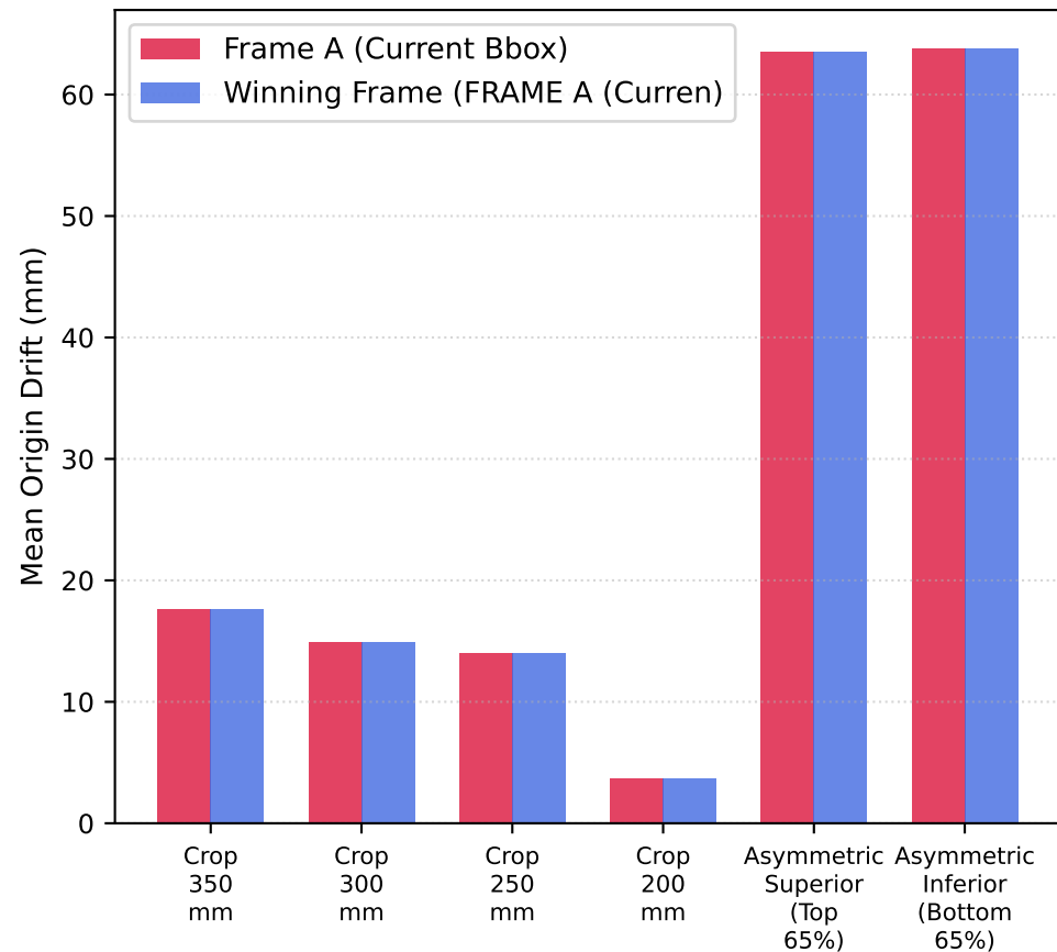
B: Drift Comparison Across Synthetic Crops
