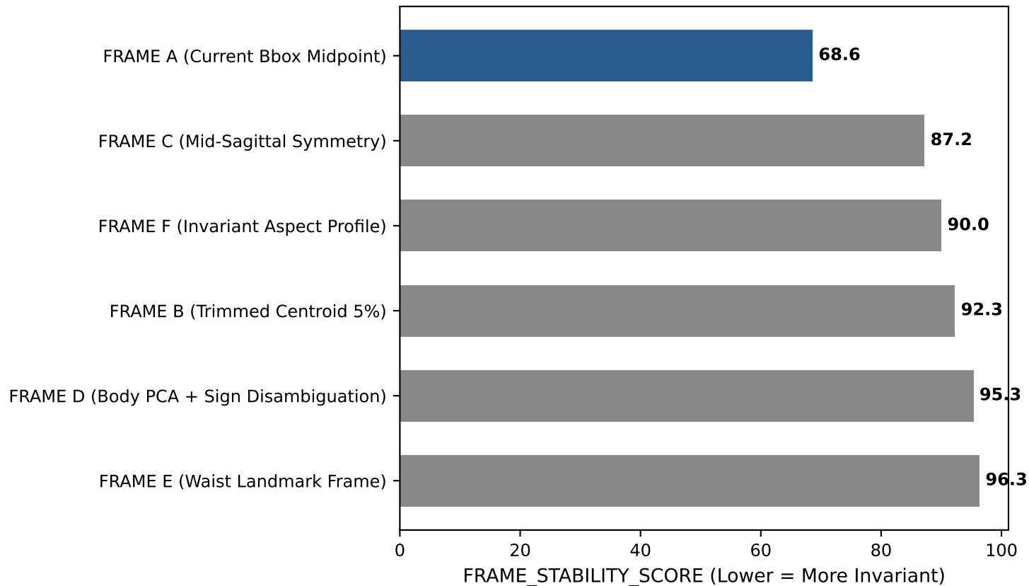
A: Canonical Frame Stability Ranking (V3 Validation)
