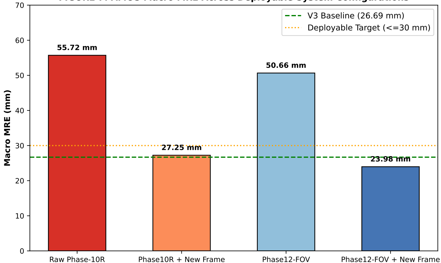
FIGURE 7: AMOS Macro MRE Across Deployable System Configurations
