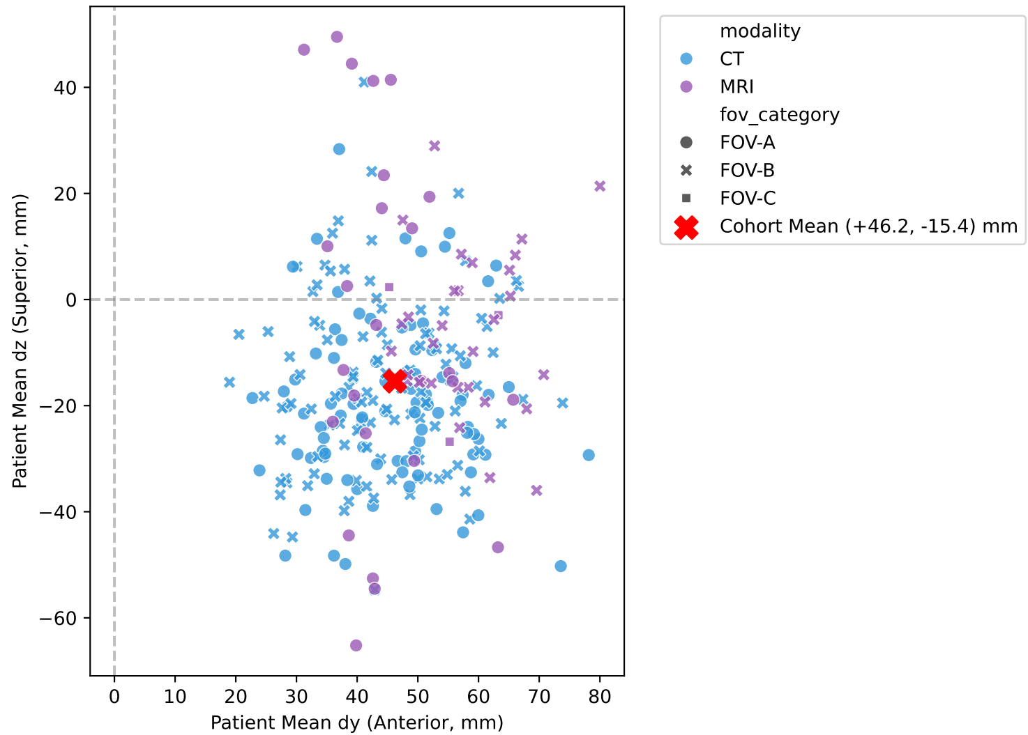
Patient-Level Mean Displacement Vectors (Anterior-Posterior vs Superior-Inferior)
