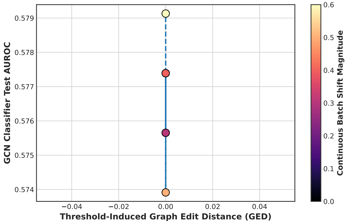
Test 6: GNN Generalization Collapse strictly vs. Threshold-Induced GED
