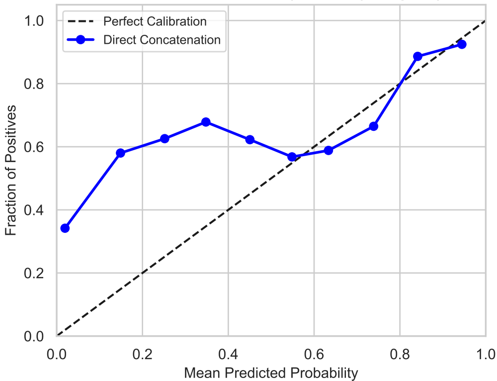
Model Calibration Curve (Reliability Diagram)
