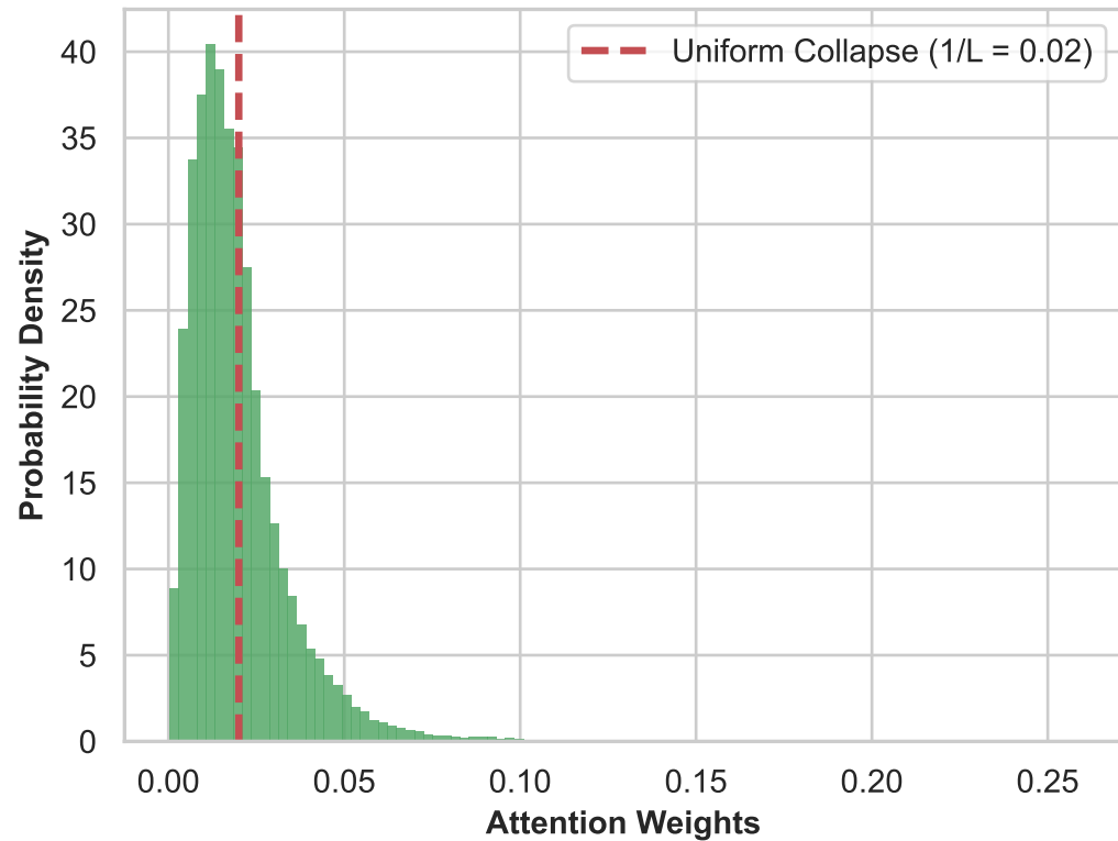
B. Cross-Attention Softmax Collapse
