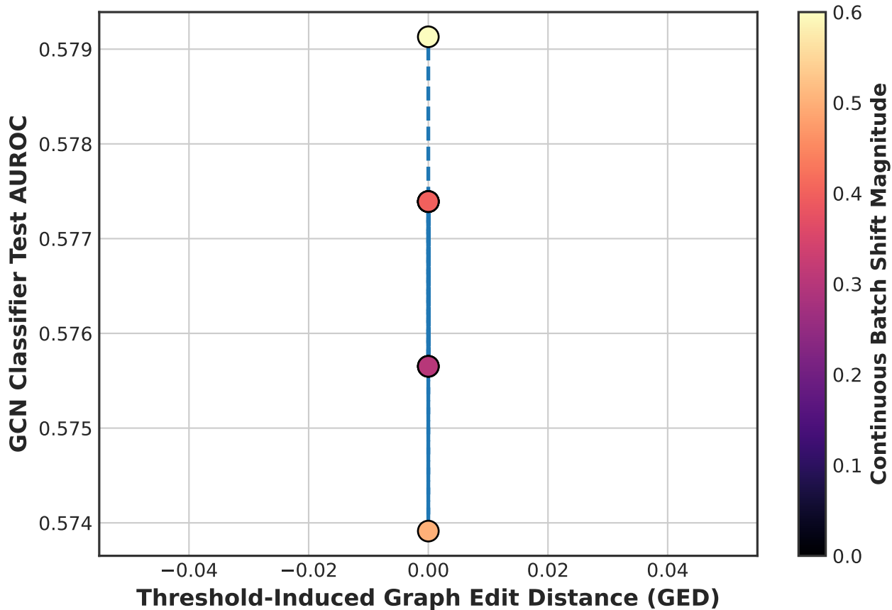
Figure 6: GNN Generalization Collapse strictly vs. Threshold-Induced GED
