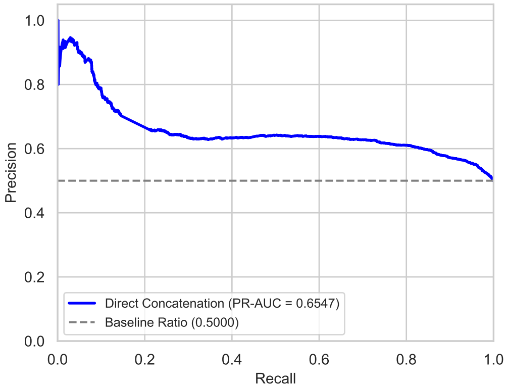
Precision-Recall (PR) Curve
