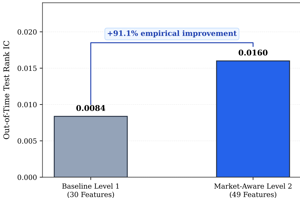
Figure 5. Paired Out-of-Time Rank IC Comparison (H = 5 Days)
