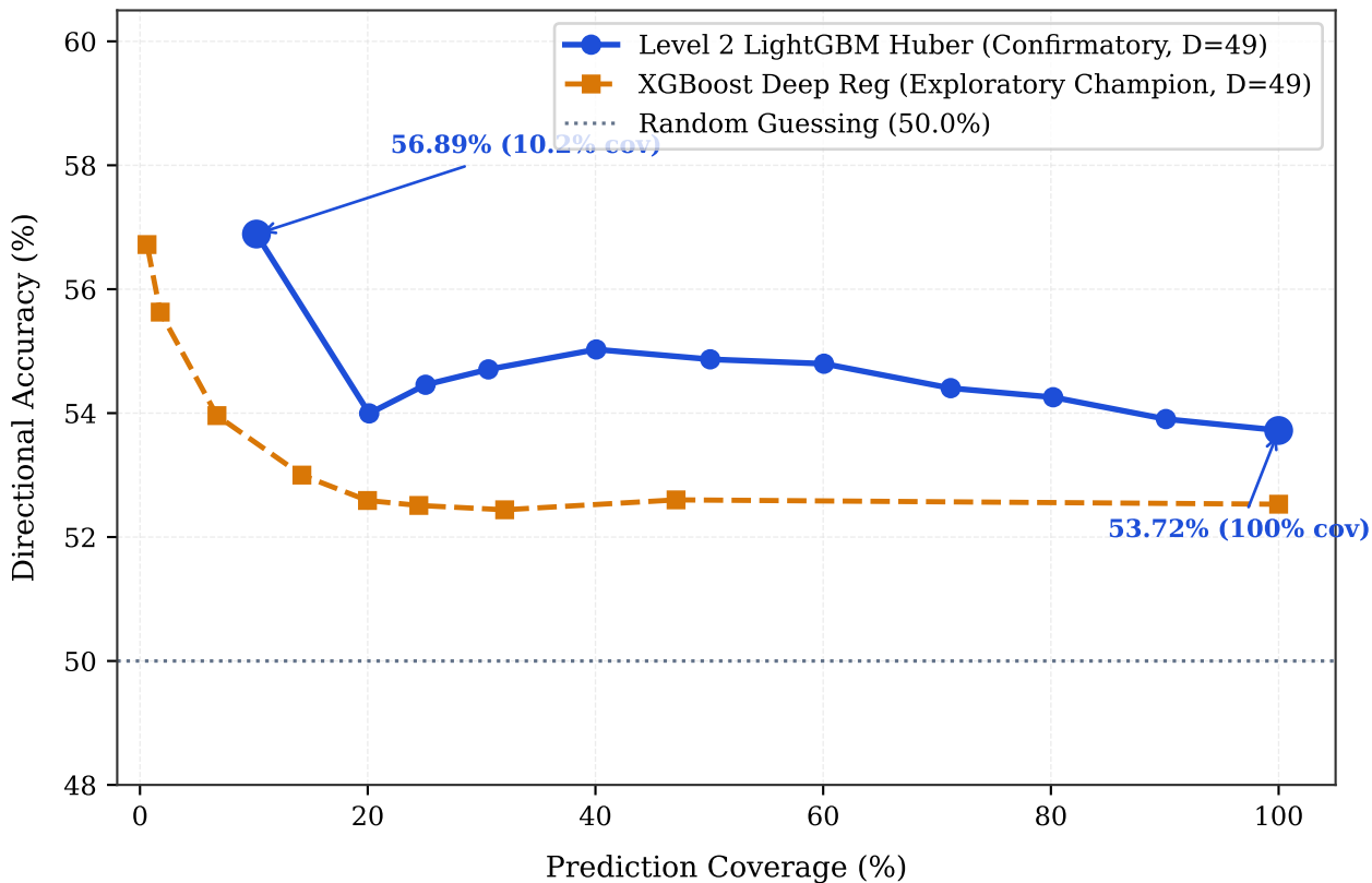
Figure 6. Selective Directional Accuracy as a Function of Coverage Tier
