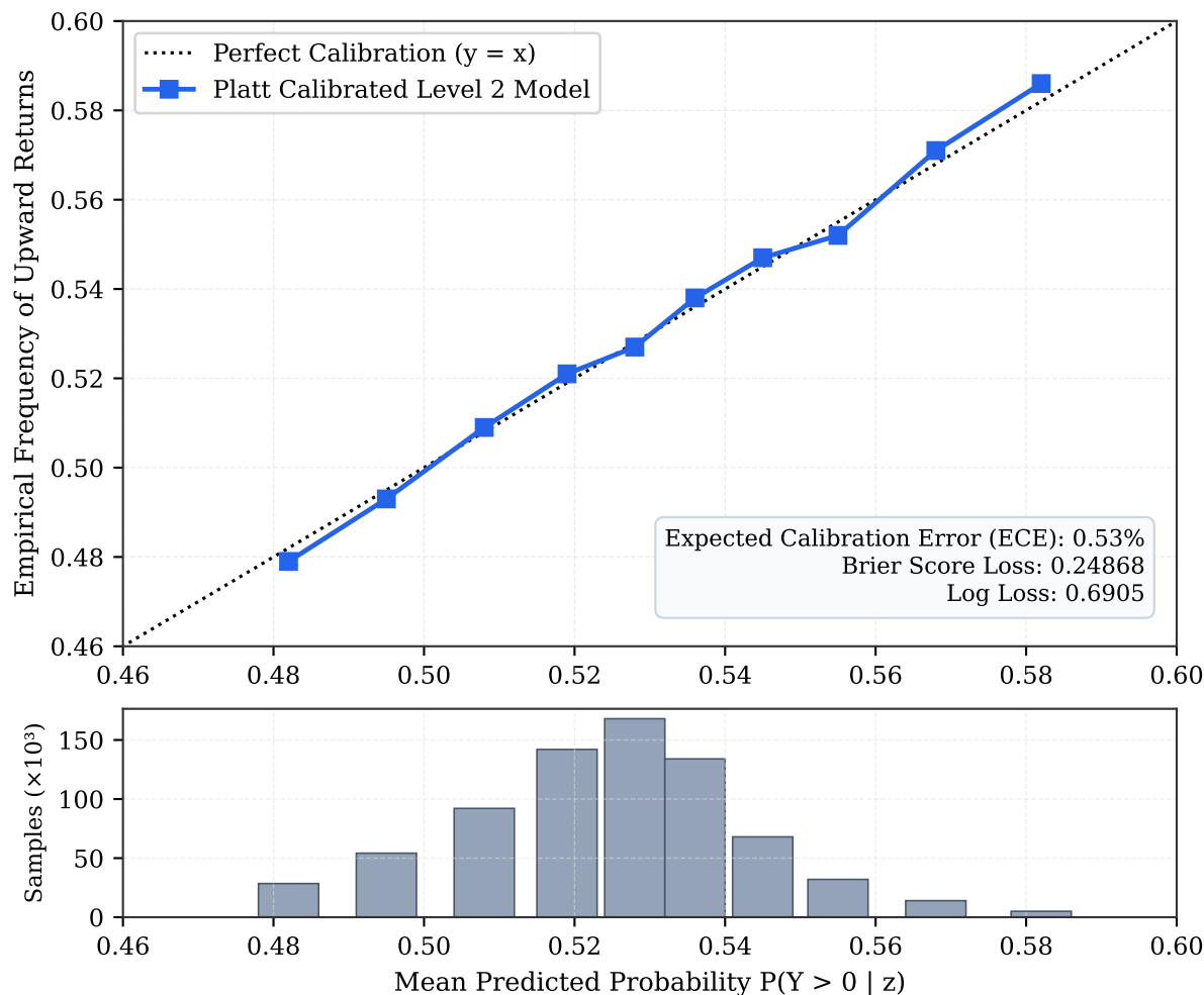
Figure 8. Out-of-Time Probability Calibration Diagnostics (Platt Logistic Scaling)
