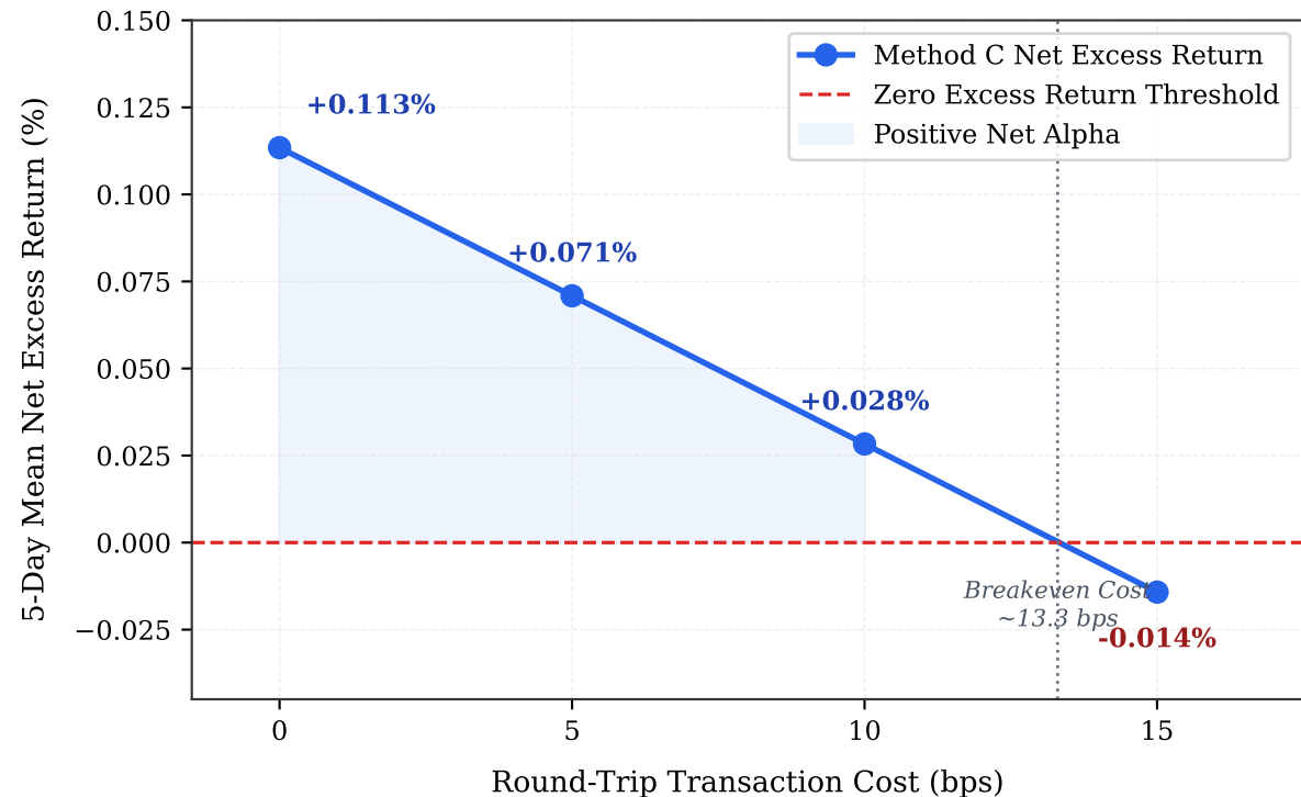
Figure 12. Method C Out-of-Time Net Excess Return Under Transaction Costs
