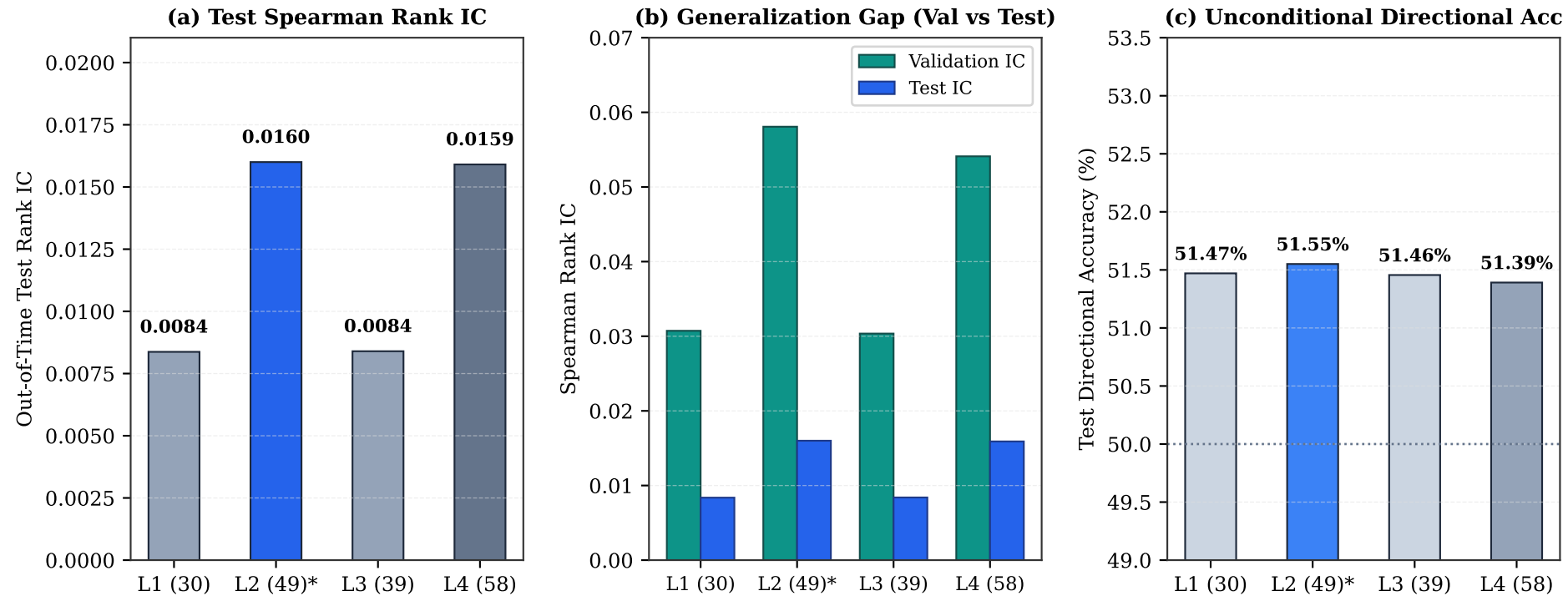
Figure 13. Comprehensive Performance Comparison Across the 4 Feature Tiers
