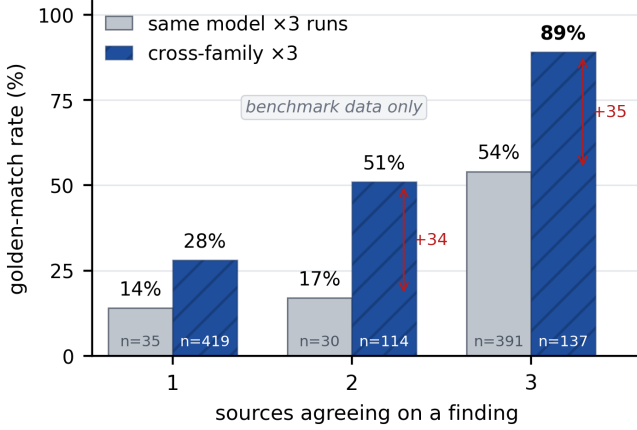
Fig. 2. Benchmark data only (injected-defect ground truth). Agreement predicts truth only when the agreeing sources are independent . Repeating one model three times barely improves on a single run until full recurrence, and saturates at that model’s error ceiling (54%); three independent families reach 89%. The gap at equal depth—+34 and +35 points—is the correlated-error mechanism made visible. This benchmark relationship reaches its ecological boundary on unlabeled industrial code, where correctness labels are absent (Section IV-H).
