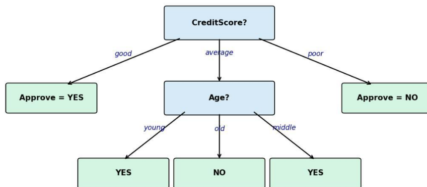
Decision Tree for Loan Approval (ID3 / Information Gain)
