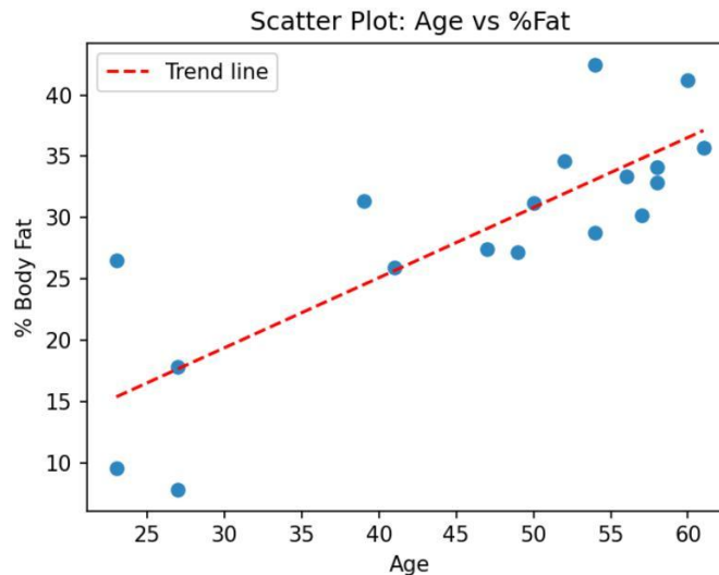
Scatter plot of Age vs %Fat ( r = 0.818 ).
