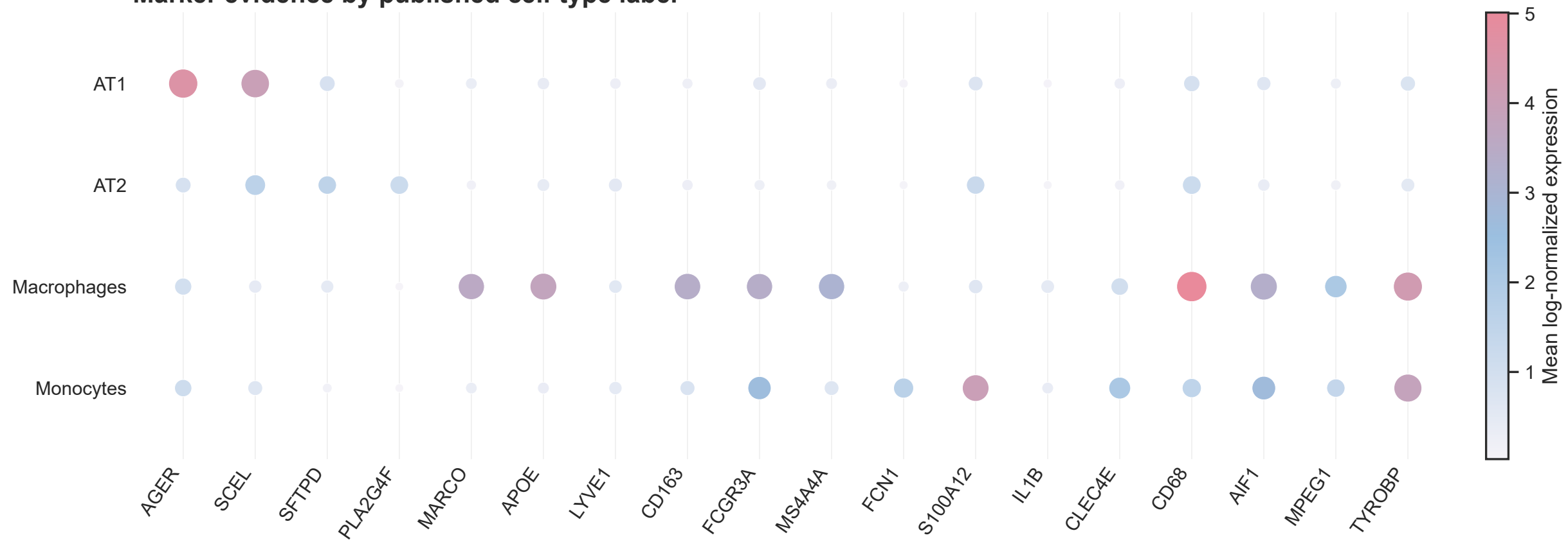
Marker expression by published cell-type label
