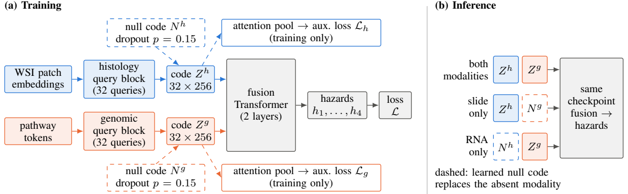
Fig. 1. PathQ-Former is trained for missingness and served from one checkpoint. (a) Training. The WSI patch embeddings and the pathway tokens are each read by a block of 32 learned queries, giving codes Z^h, Z^g \in \mathbb{R}^{32 \times 256} that a two-layer fusion Transformer maps to four discrete-time hazards and the survival loss \mathcal{L} . With probability p = 0.15 per sample, modality dropout replaces a present code by its learned null code N^h or N^g (dashed), and auxiliary survival losses \mathcal{L}_h and \mathcal{L}_g on the attention-pooled codes make each branch prognostic on its own (training only). (b) Inference. Patients with both modalities, a slide only or RNA only enter the same checkpoint; the code of the absent modality is replaced by its null code and nothing else changes.
