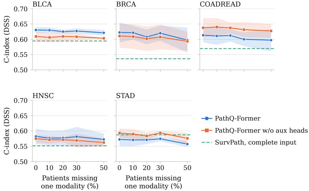
Fig. 3. C-index of PathQ-Former and of its variant without auxiliary heads (‘w/o aux heads’ in the legend; 20 epochs) when 0–50% of validation patients are missing one modality at random (mean of five random draws per fold). Lines: mean over three seeds of the five-fold mean; bands: \pm 1 sd over seeds. Dashed line: SurvPath with complete inputs (three-seed mean). With half the patients missing a modality the fused C-index changes by at most 0.025 (BRCA).
