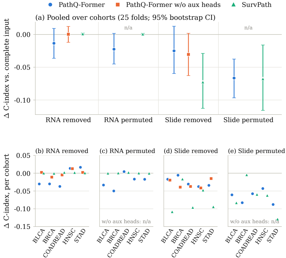
Fig. 2. Change in C-index of the same 20-epoch checkpoint when one test-time input is removed or permuted across validation patients, relative to its complete-input evaluation. In the legend, ‘w/o aux heads’ is the variant without auxiliary heads. SurvPath receives the training-mean gene vector or patch embedding for a removed input; PathQ-Former uses its learned null codes. (a) Pooled over the five cohorts: per (cohort, fold) the change is averaged over three seeds, then the mean and 95% bootstrap confidence interval over the 25 folds are shown (10,000 resamples of folds). (b)–(e) The same quantity per cohort (mean over five folds). The variant without auxiliary heads was not evaluated under permutation (n/a).
