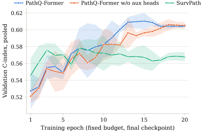
Fig. S1. Validation C-index per training epoch under the 20-epoch budget, pooled over all cohorts and folds, for PathQ-Former, its variant without auxiliary heads ('w/o aux heads') and SurvPath: mean over three seeds, \pm 1 sd band over seeds. All results use the final epoch; the curves only set the budget.
