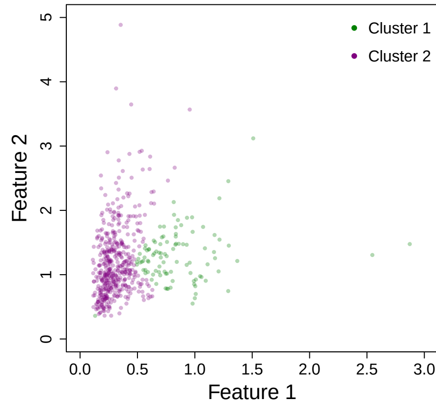
Clustering result
