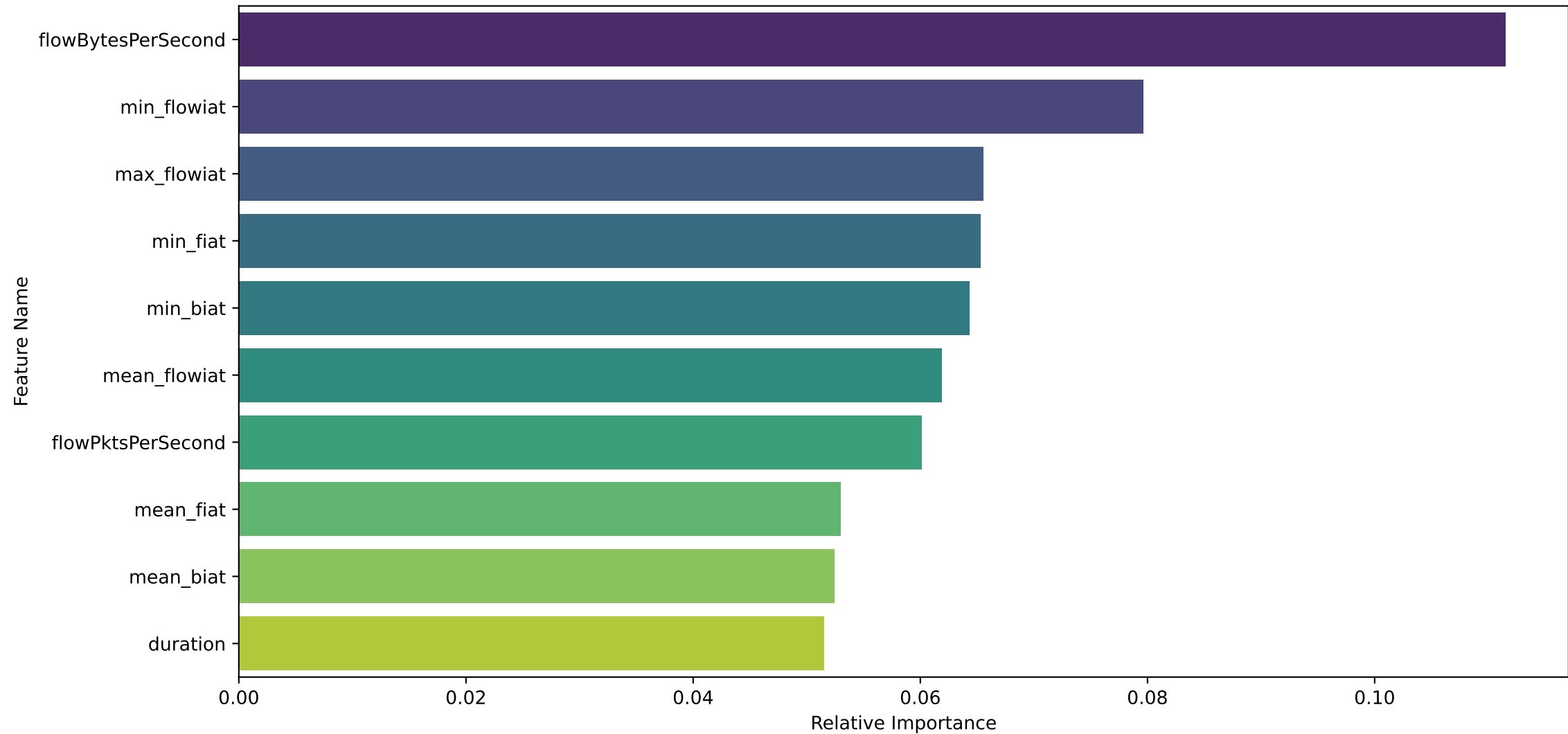
Top 10 Most Important Network Flow Features
