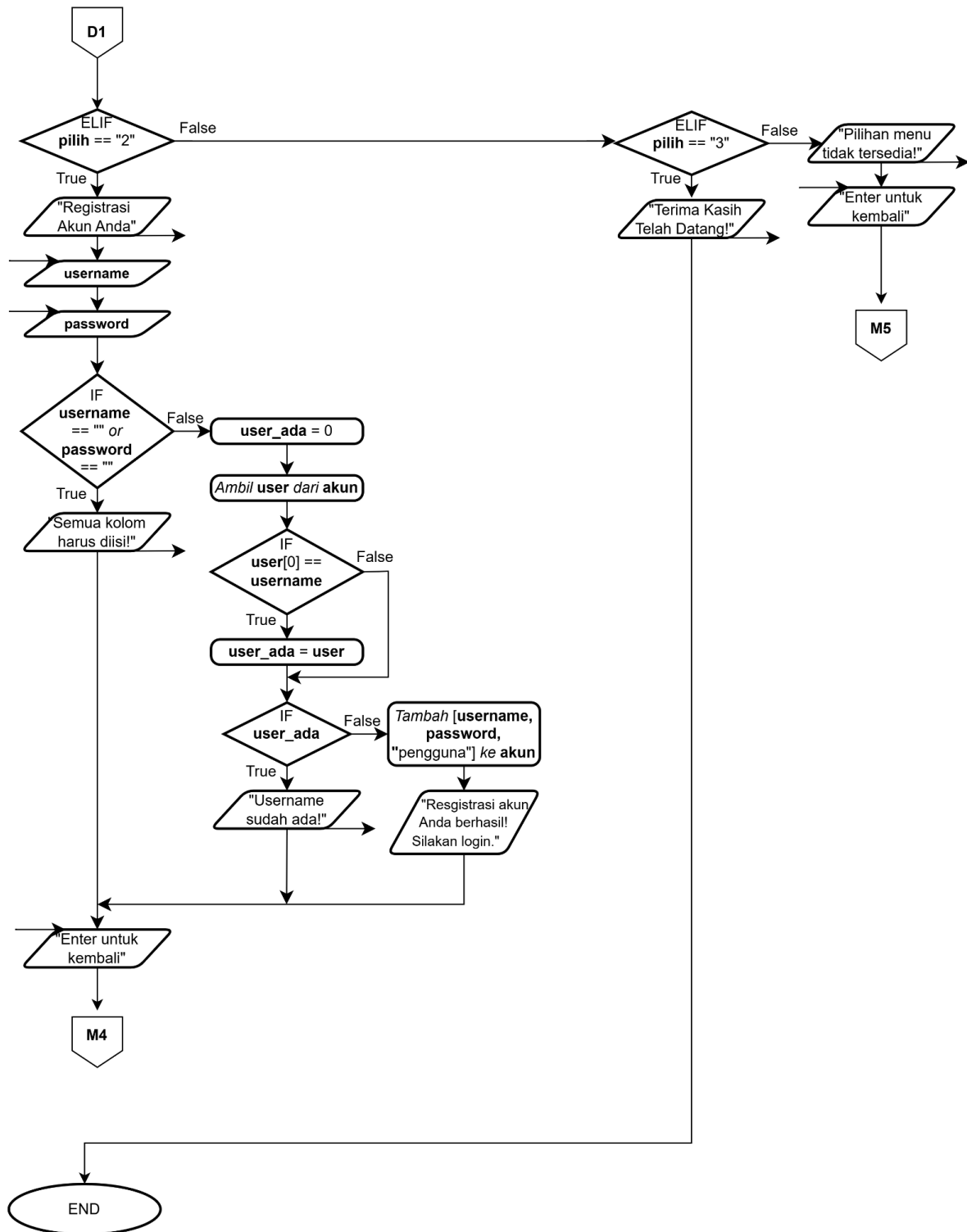
Diagram 1.5. Flowchart Program Halaman 5
