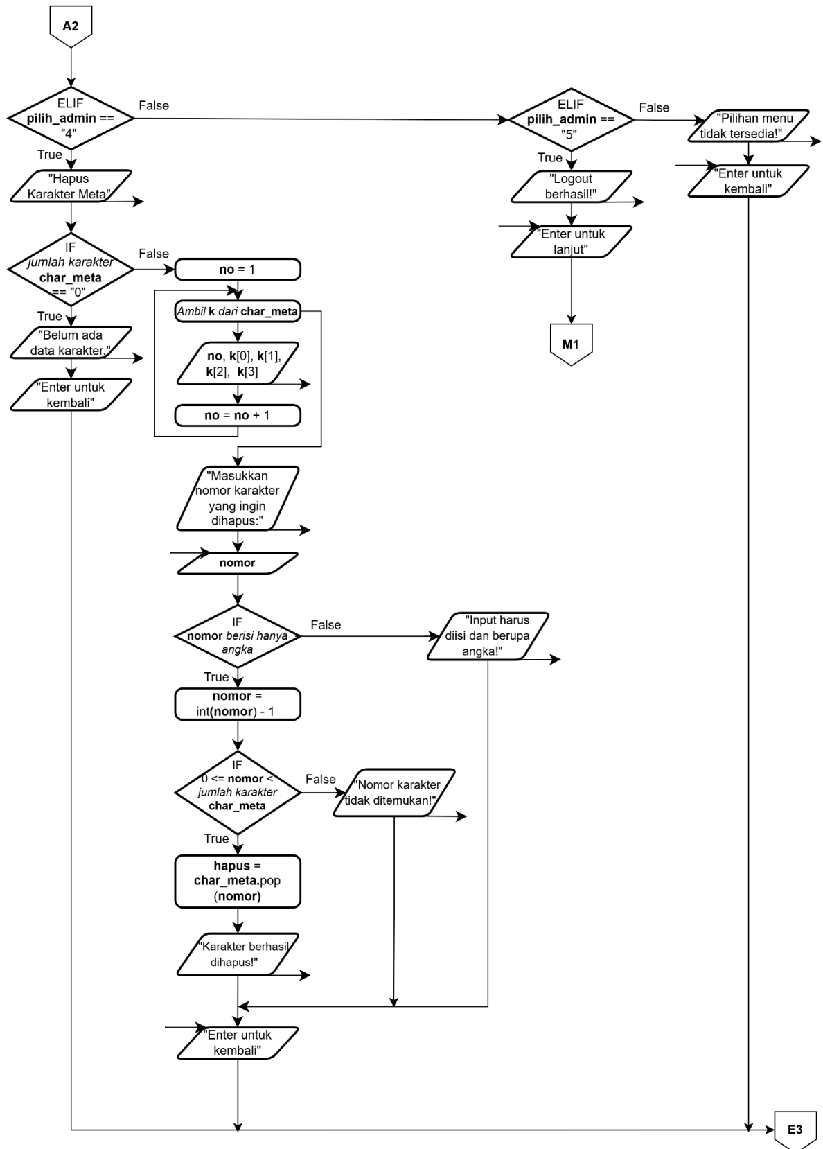
Diagram 1.3. Flowchart Program Halaman 3
