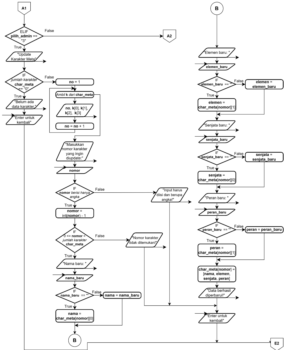
Diagram 1.2. Flowchart Program Halaman 2
