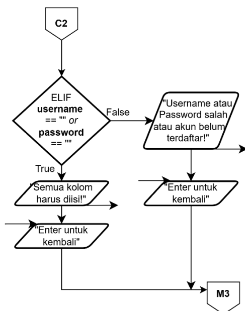
Diagram 1.4. Flowchart Program Halaman 4
