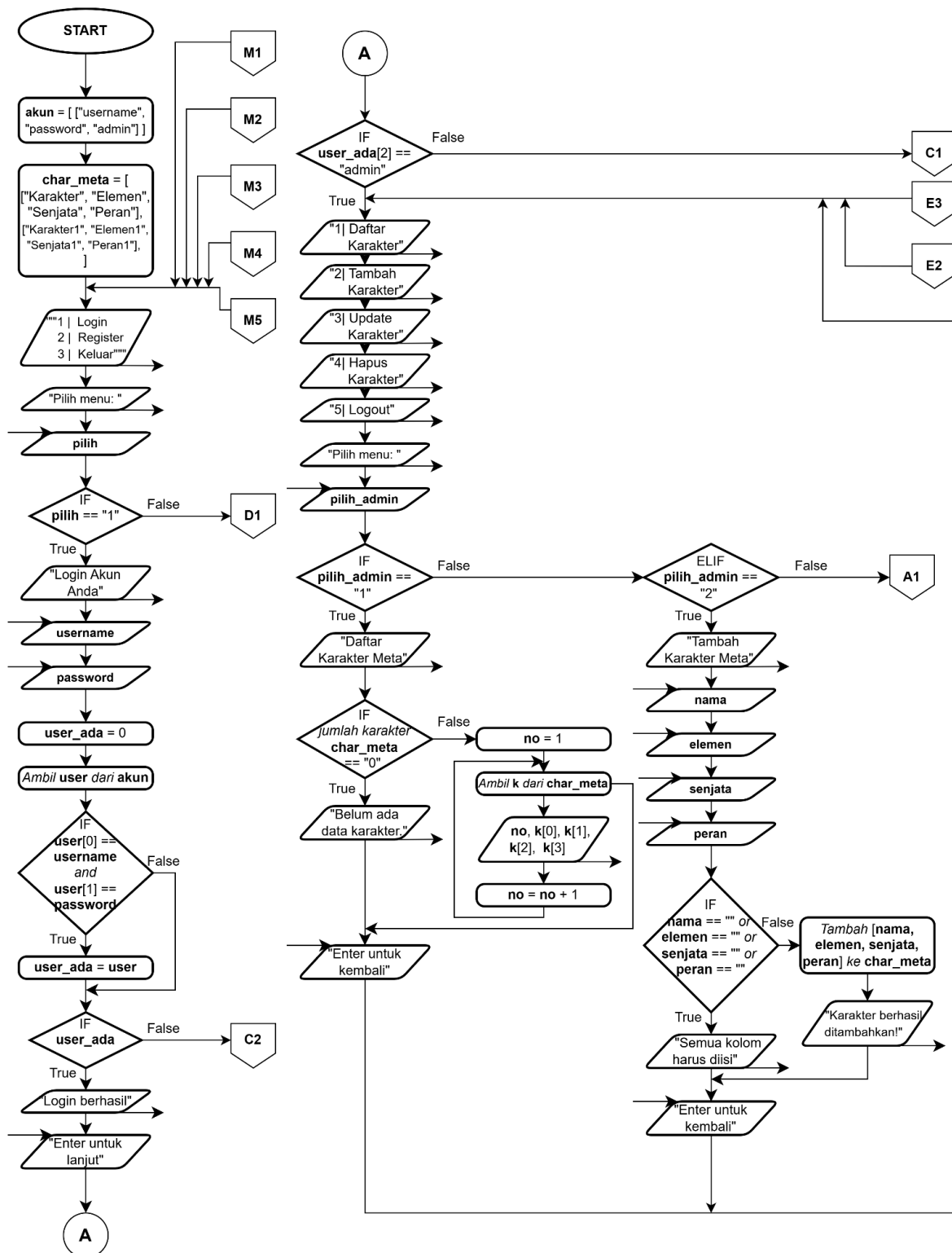
Diagram 1.1. Flowchart Program Halaman 1
