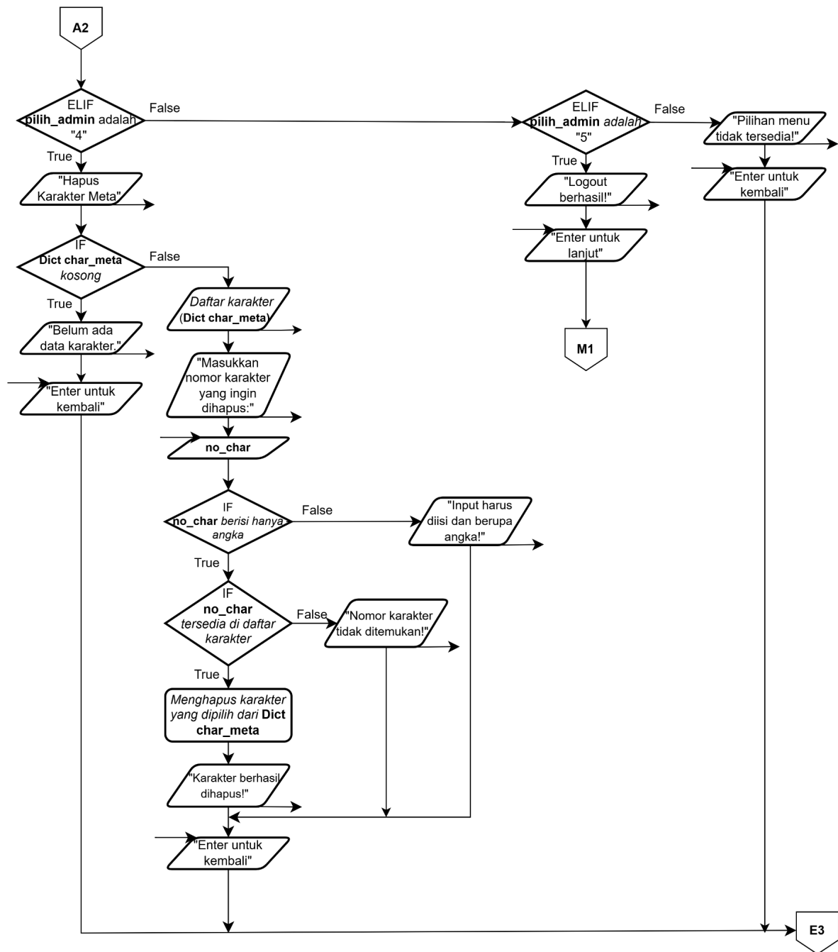
Diagram 1.3. Flowchart Program Halaman 3
