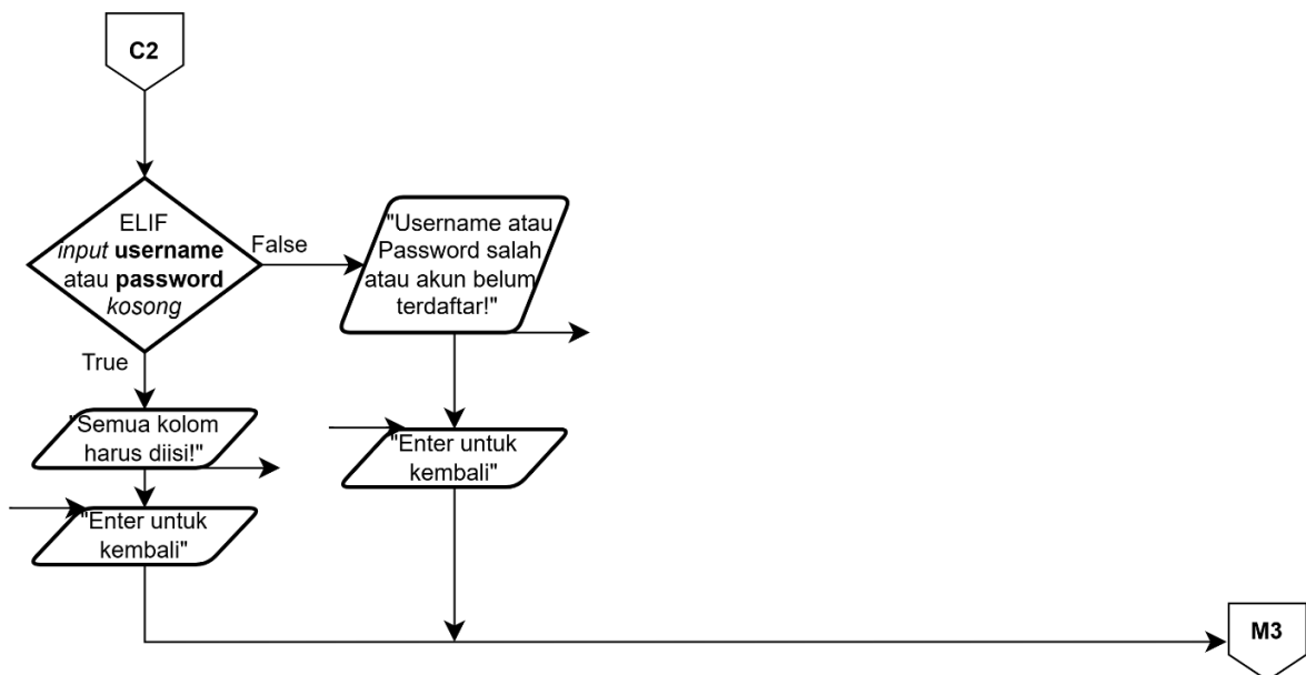
Diagram 1.4. Flowchart Program Halaman 4
