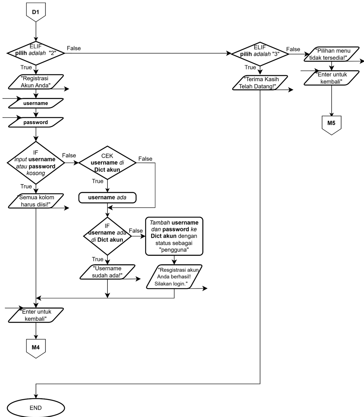
Diagram 1.5. Flowchart Program Halaman 5
