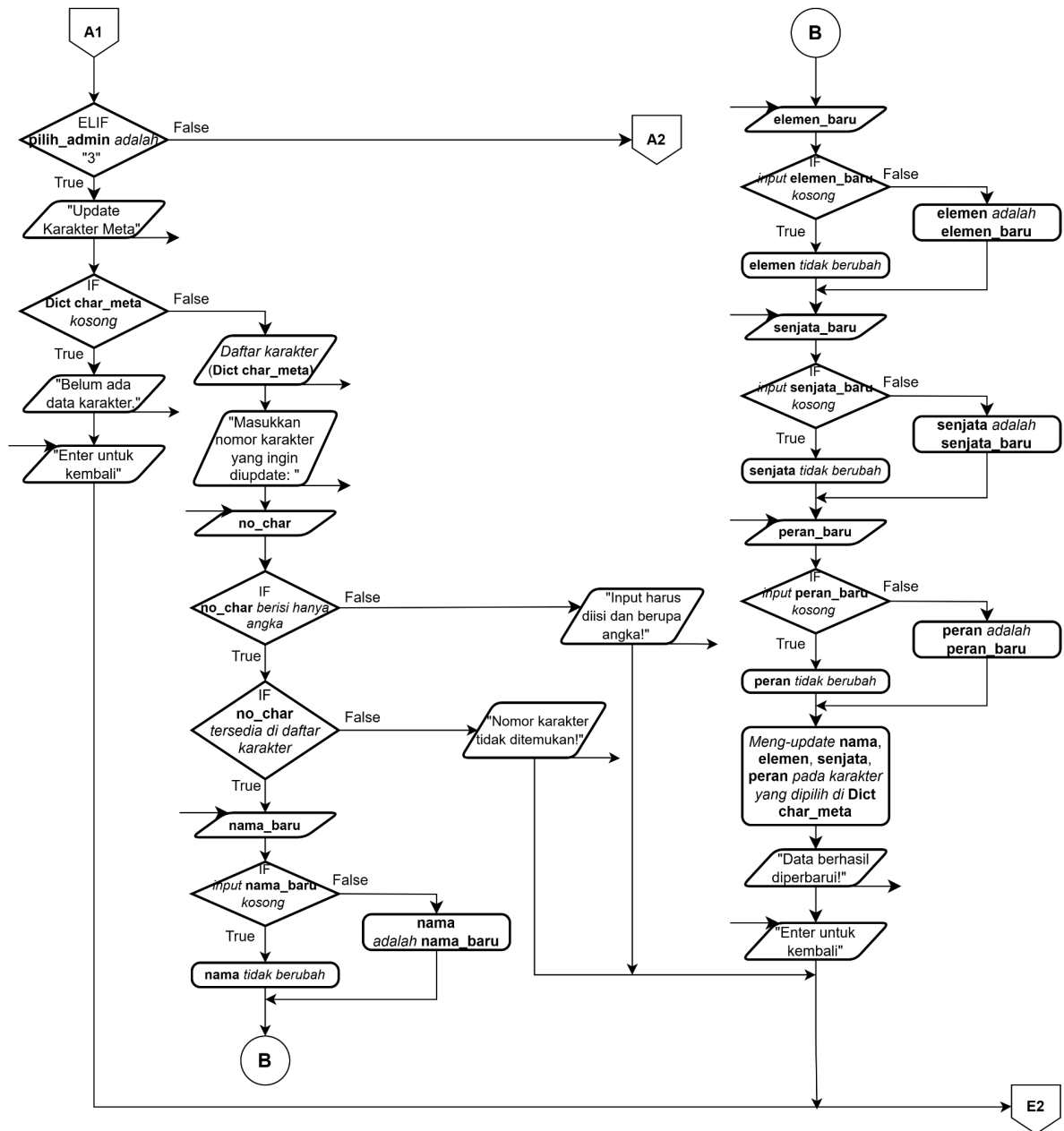
Diagram 1.2. Flowchart Program Halaman 2
