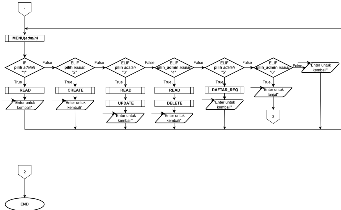
Diagram 1.6. Flowchart File Main Halaman 2
