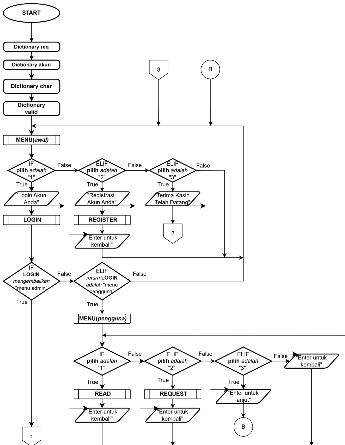
Diagram 1.5. Flowchart File Main
