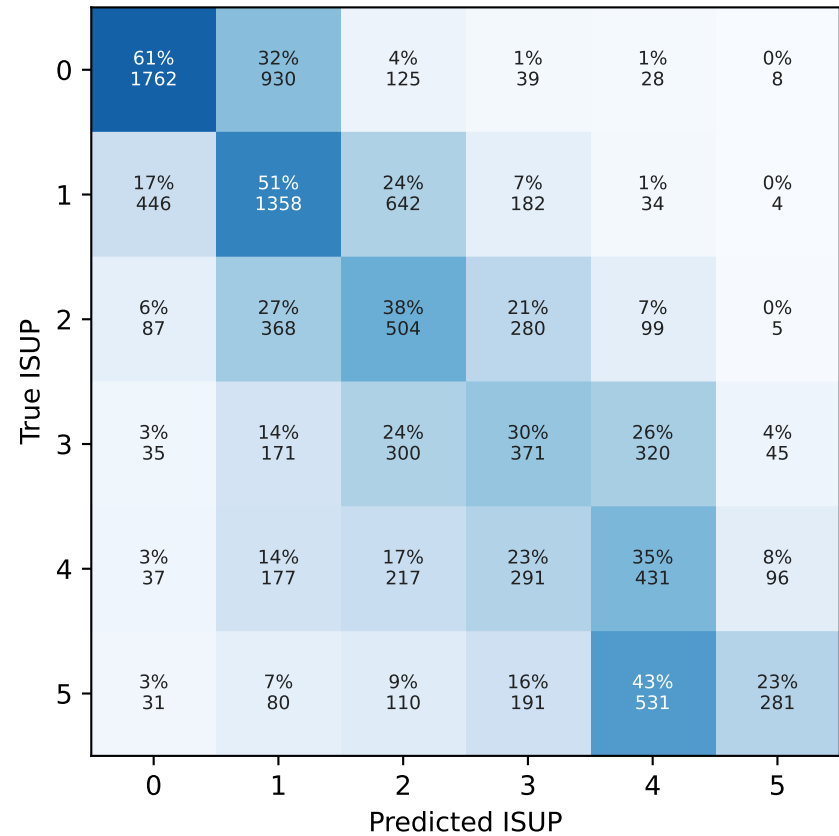
SmoothL1 recovered OOF QWK 0.7147
