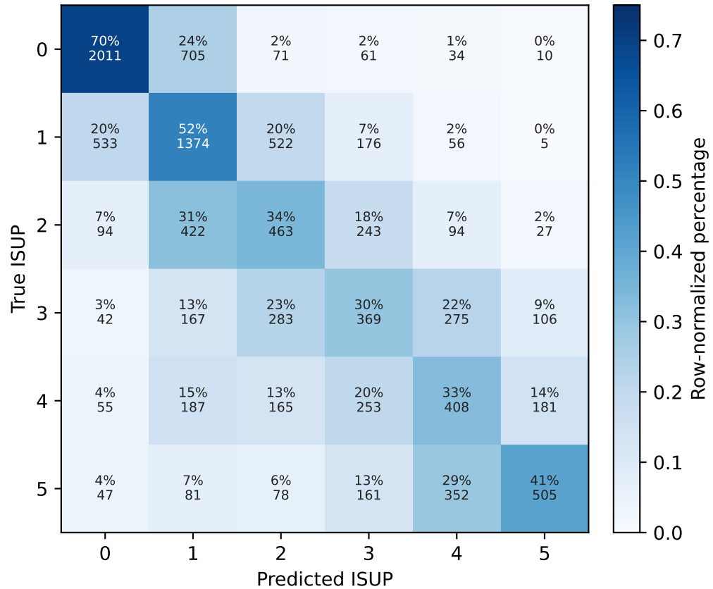
Ordinal BCE recovered OOF QWK 0.7244
