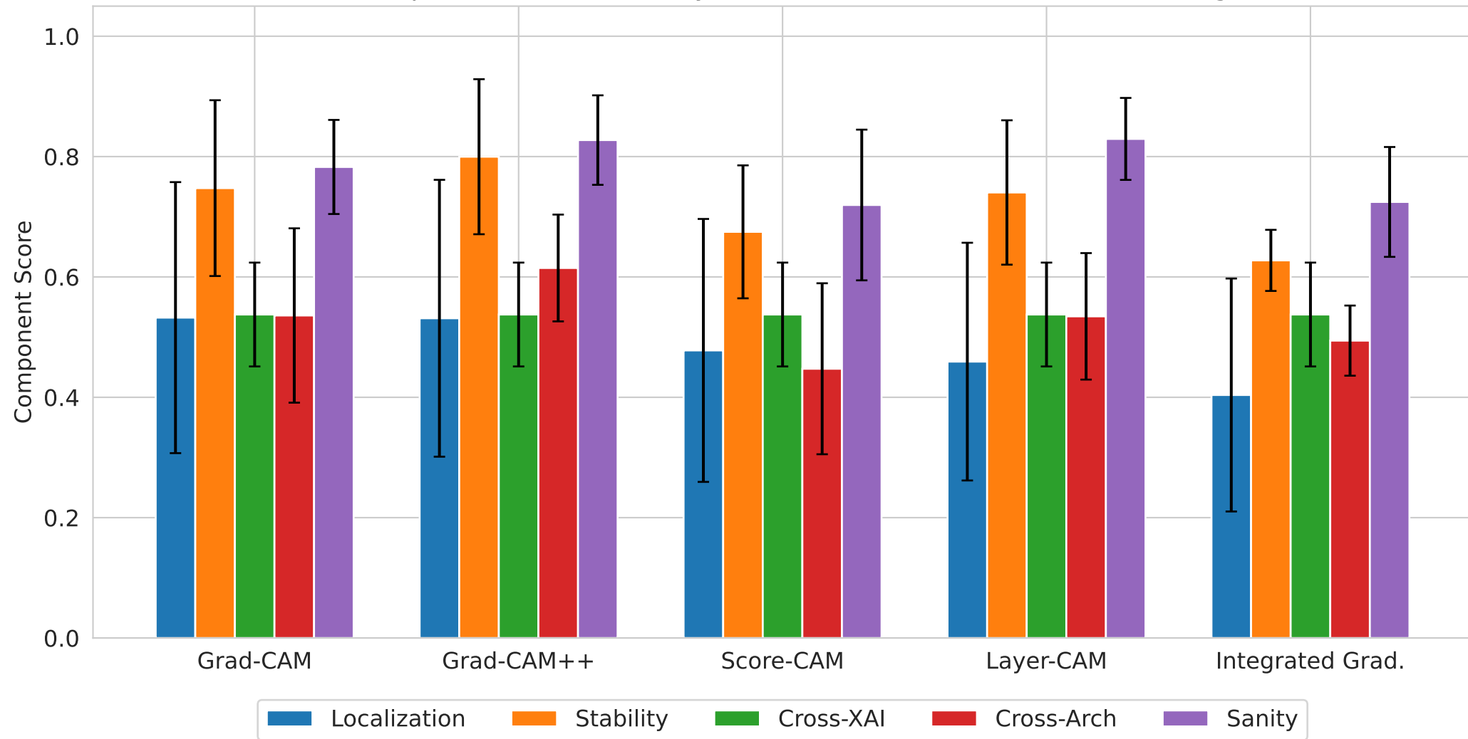
CTI Component Breakdown by XAI Method (mean \pm std across images)
