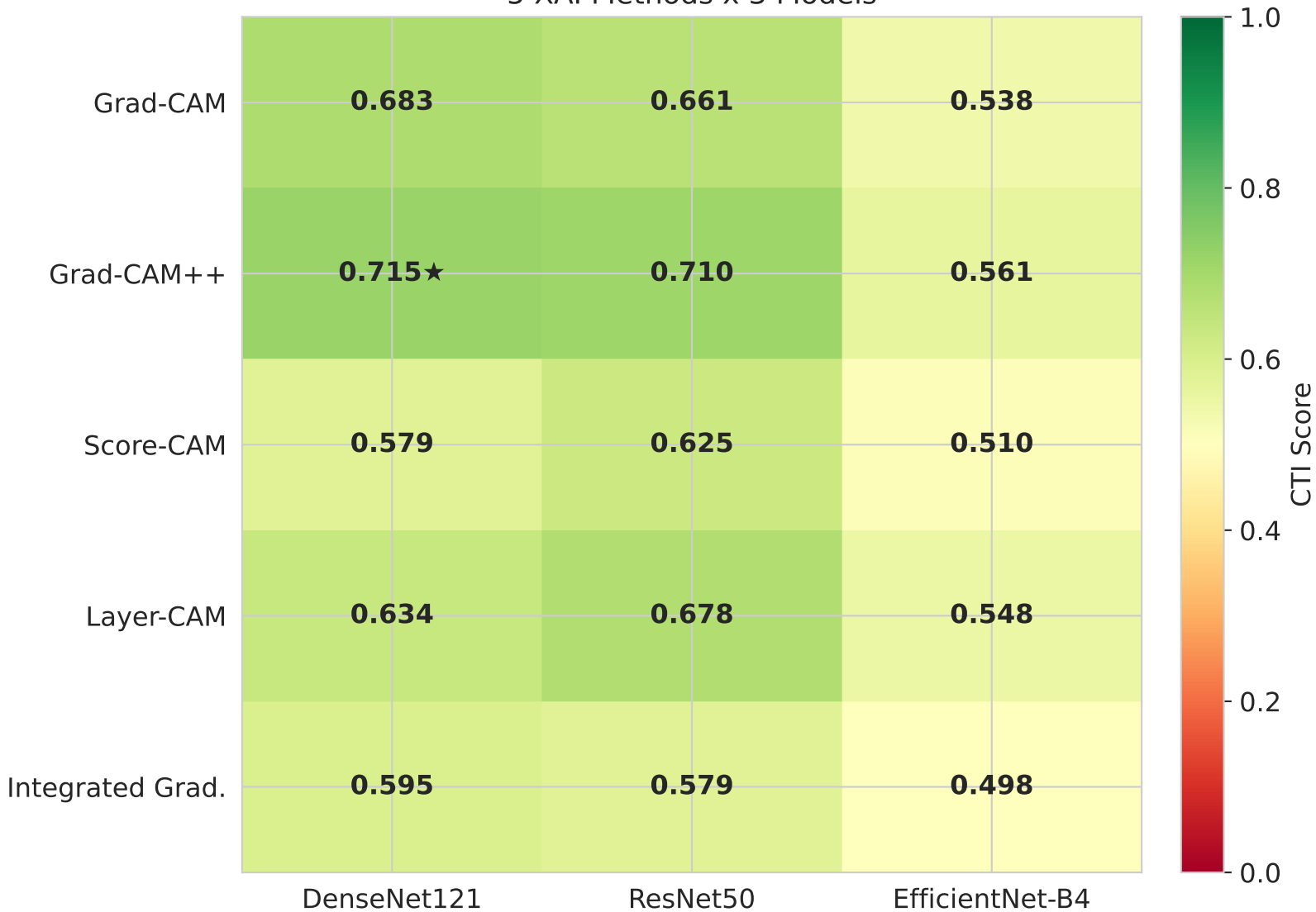
Composite Trustworthiness Index (CTI) 5 XAI Methods x 3 Models
