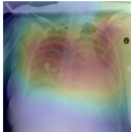
Score-CAM CTI=0.506
