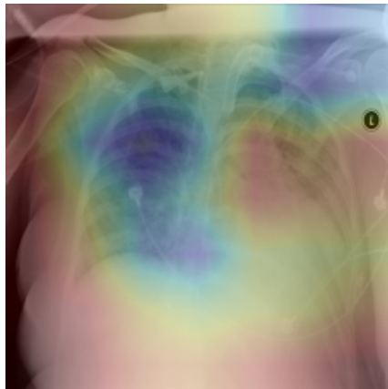
Grad-CAM CTI=0.317
