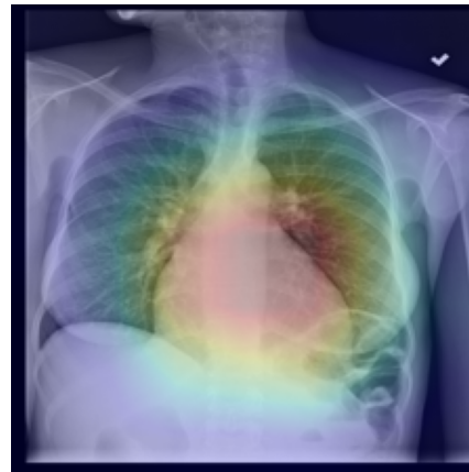
Score-CAM CTI=0.749
