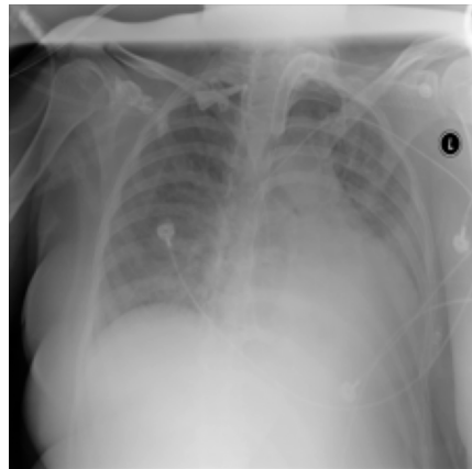
Lowest CTI 00018187_034
