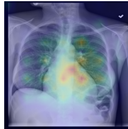
Layer-CAM CTI=0.712
