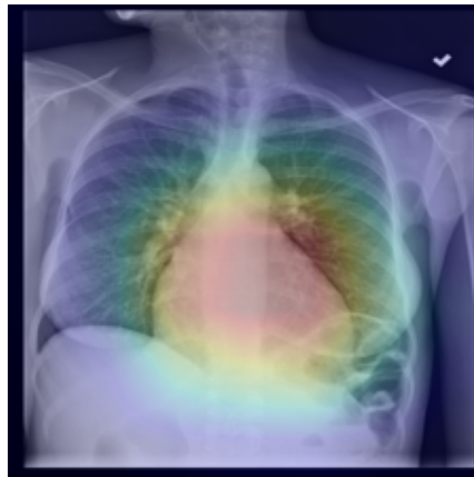
Grad-CAM++ CTI=0.794
