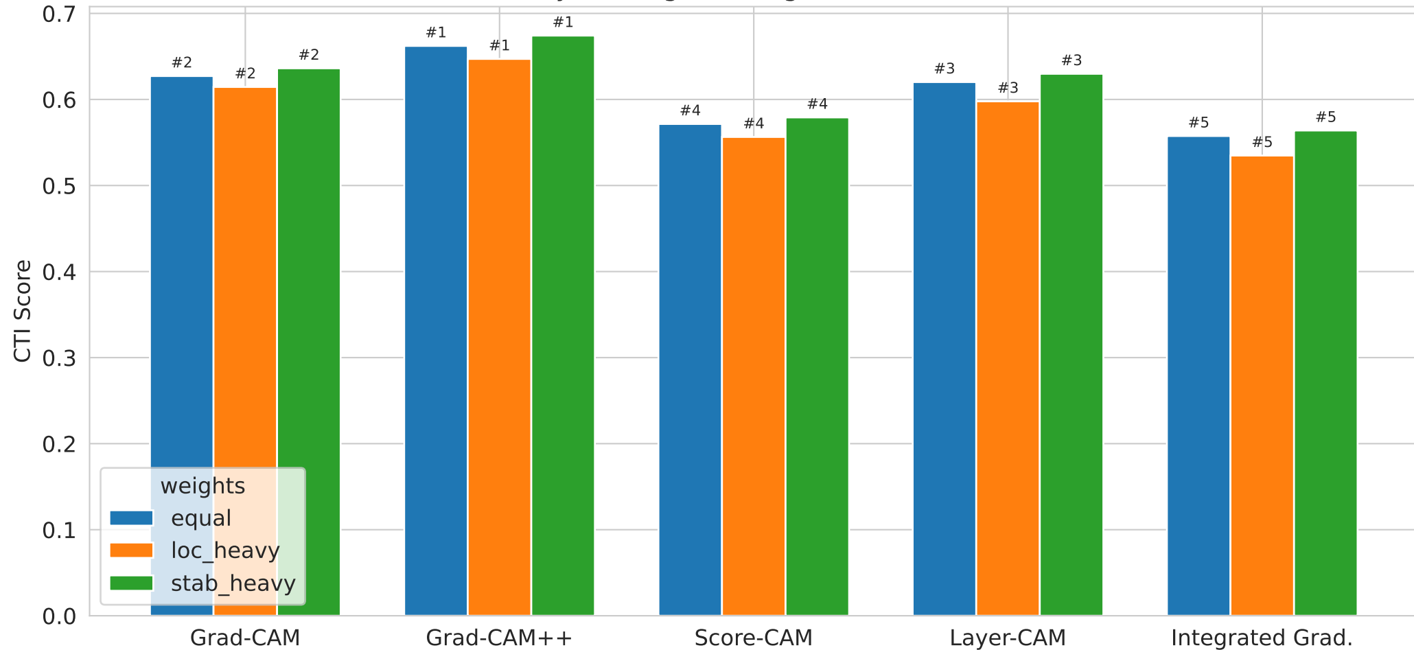
CTI Sensitivity to Weight Configuration (rank annotated)
