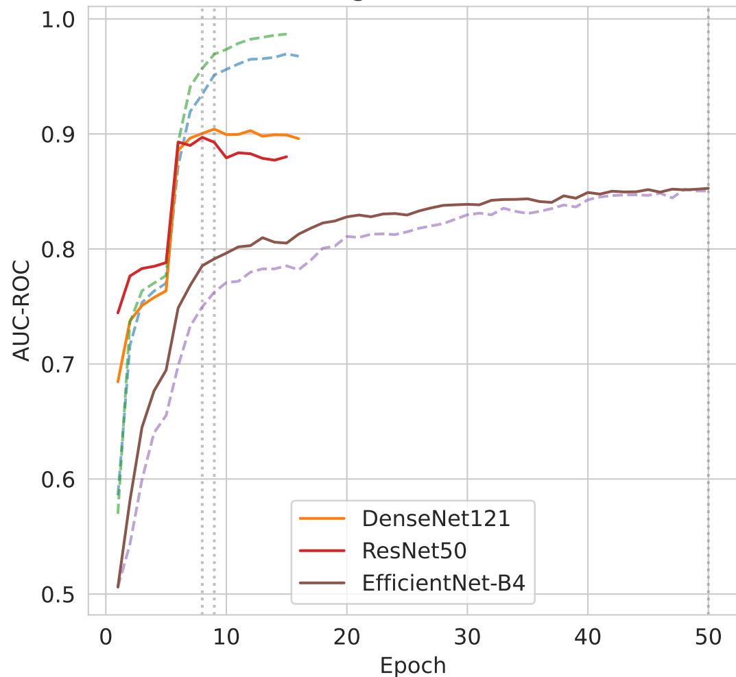
Training / Val AUC-ROC
