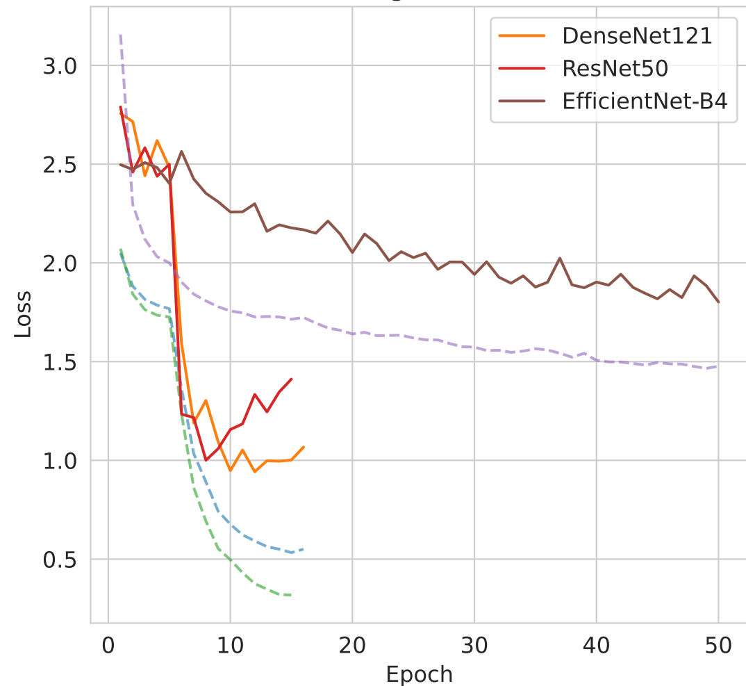
Training / Val Loss
