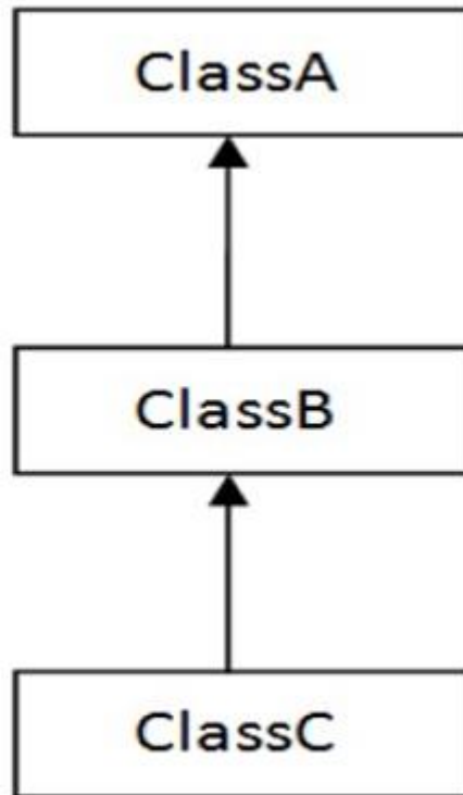
2) Multilevel
