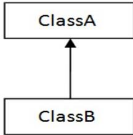
1) Single
