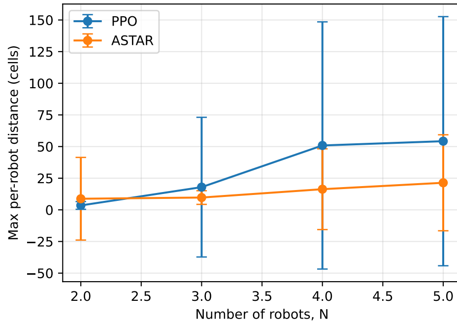
Scaling with fleet size: PPO vs A* baseline
