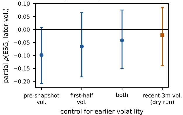
(b) the signal fades given recent volatility
