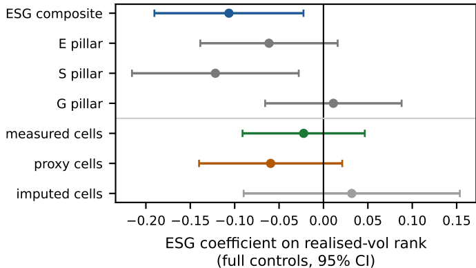
(a) which ESG data carry the signal
