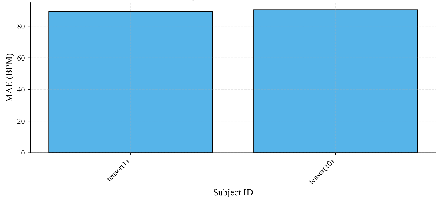
Subject-wise Performance
