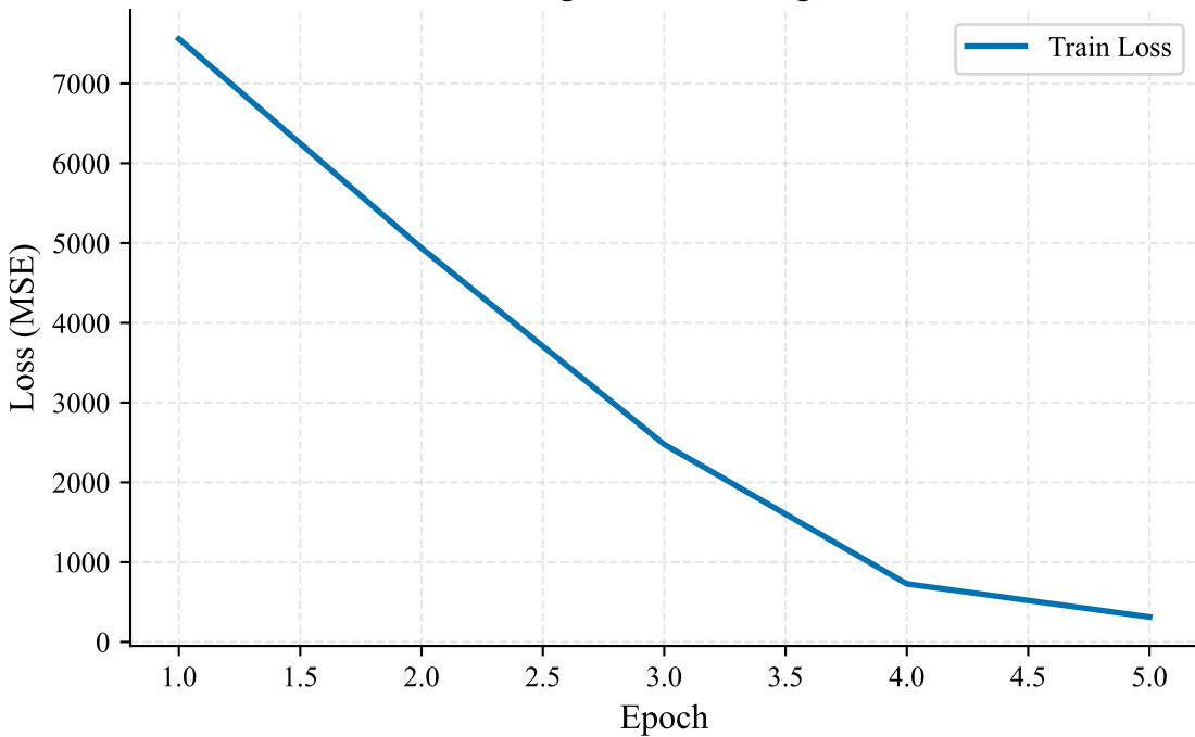
Training Loss Convergence
