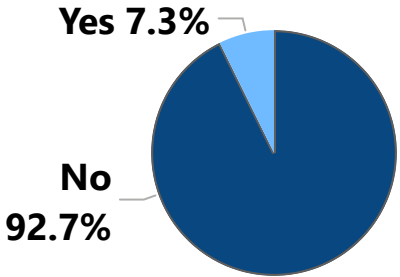
Subscription Status
