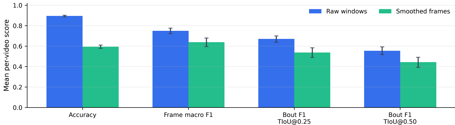
(A) Held-out performance and smoothing sensitivity
