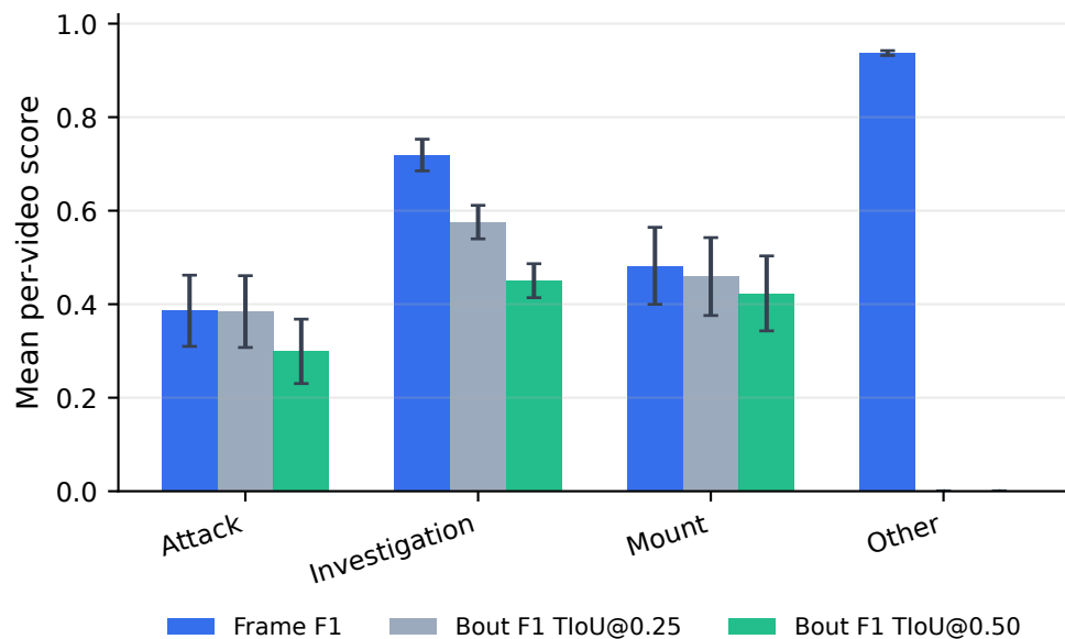
(B) Class-wise raw-window performance
