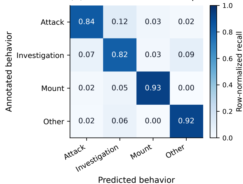
(C) Raw-window confusion profile
