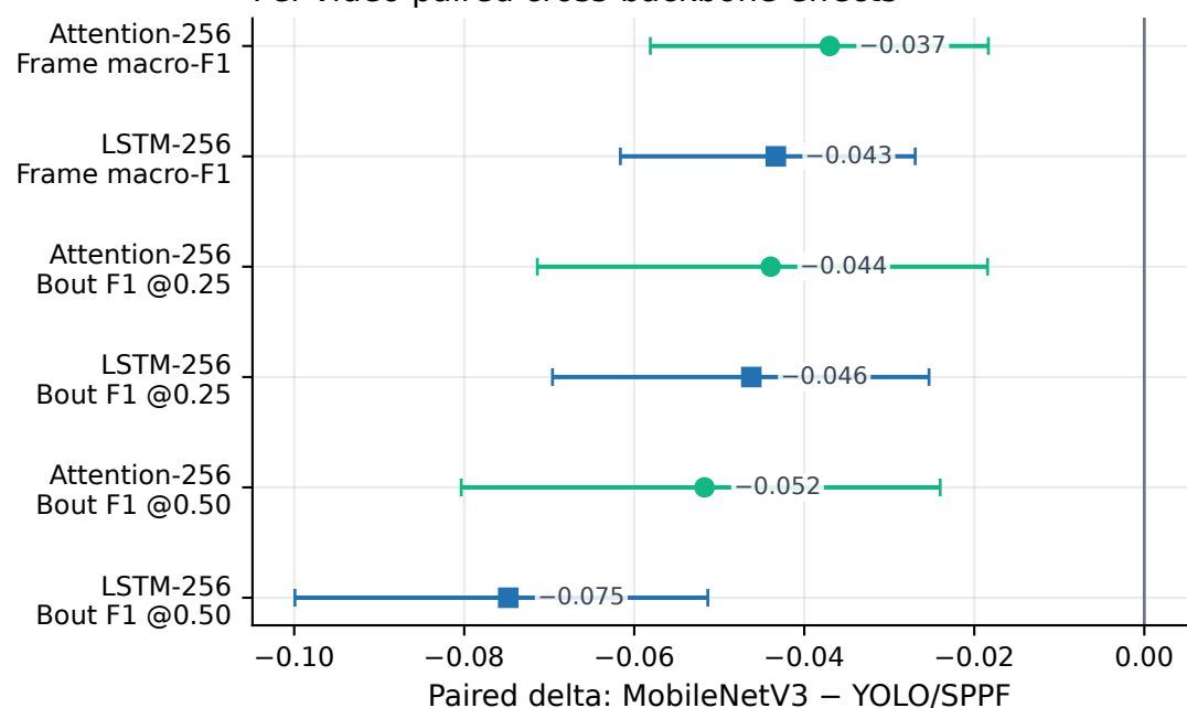
Per-video paired cross-backbone effects
