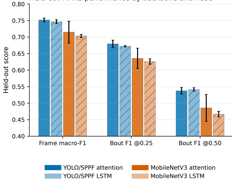
Held-out MARS performance by backbone and head
