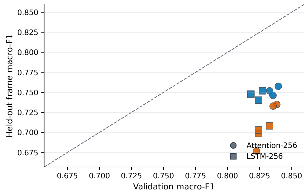
Seed-level validation vs held-out behavior
