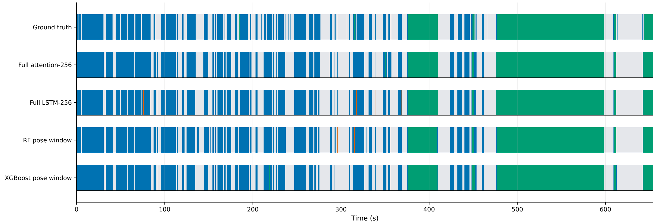
Representative MARS ethogram by model family: Mouse062_20160526_18-56-26
