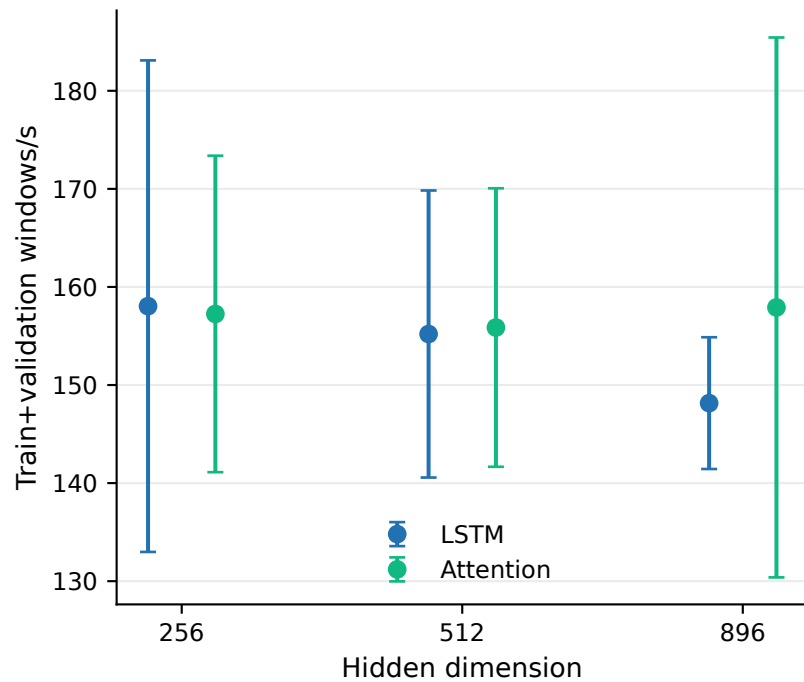
Training throughput by head/capacity
