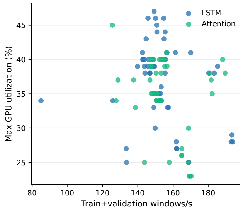
GPU utilization during training
