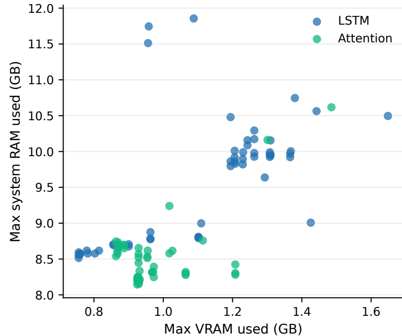
Memory footprint during training
