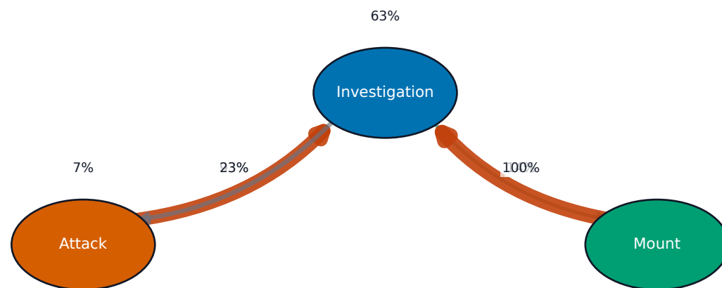
C. Bout-transition organization
