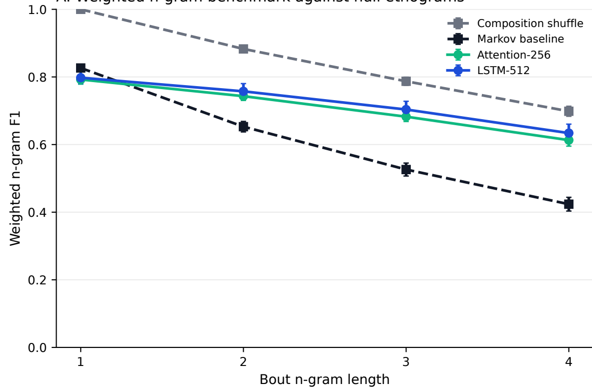
A. Weighted n-gram benchmark against null ethograms
