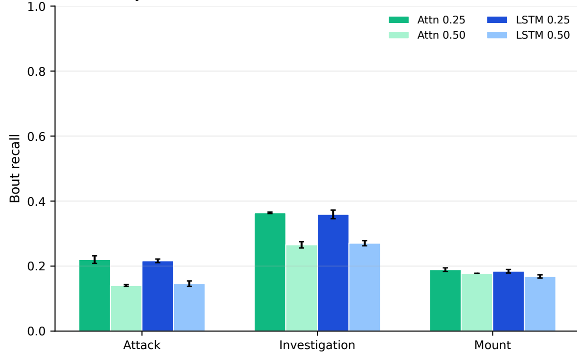
C. Boundary strictness reduces recall
