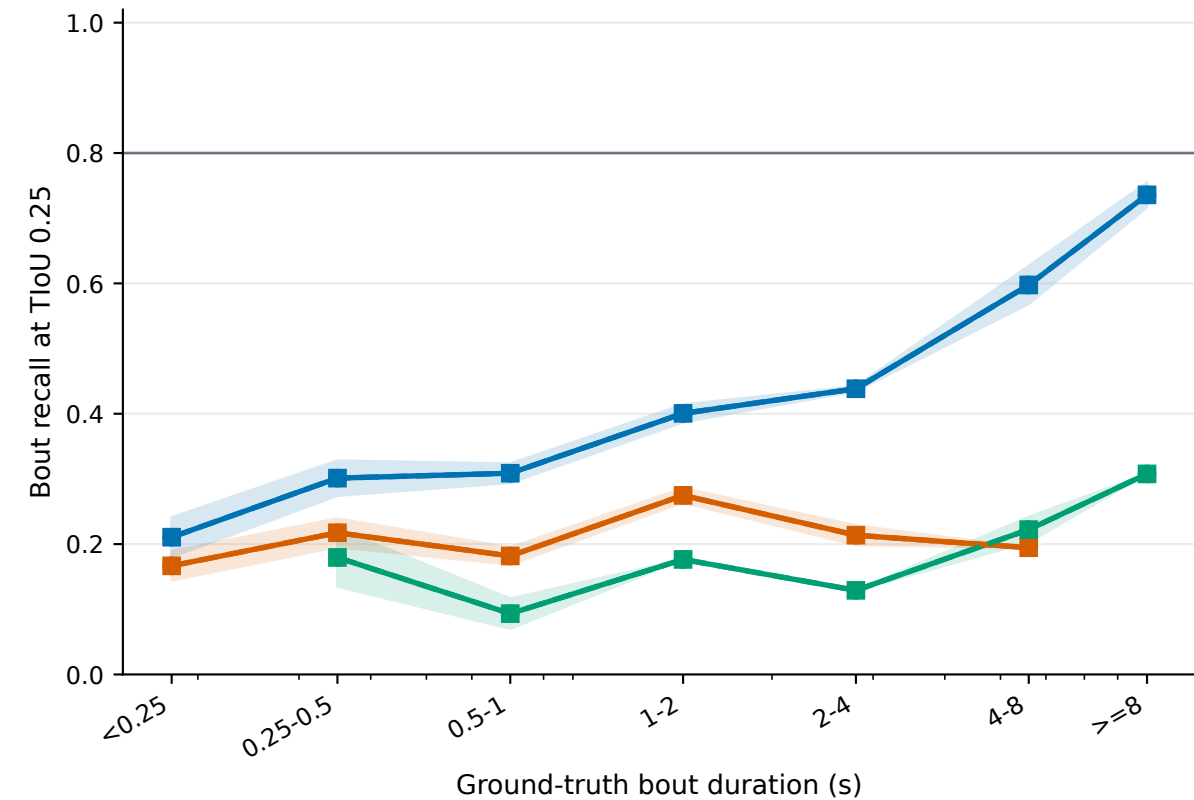
B. Operating envelope: LSTM-256
