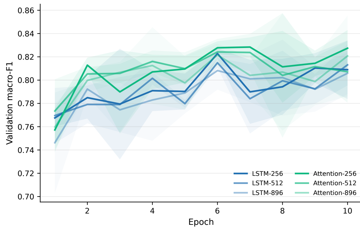
(C) Full-stream validation macro-F1
