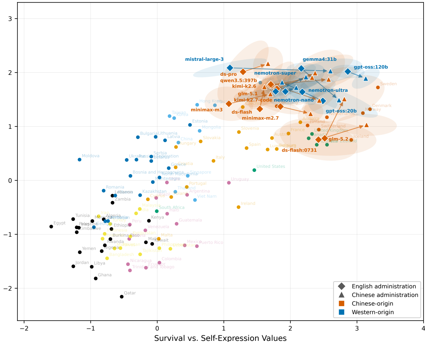
2026 frontier cohort: both administration arms (cluster-bootstrap 95% regions; arrows en→zh)
