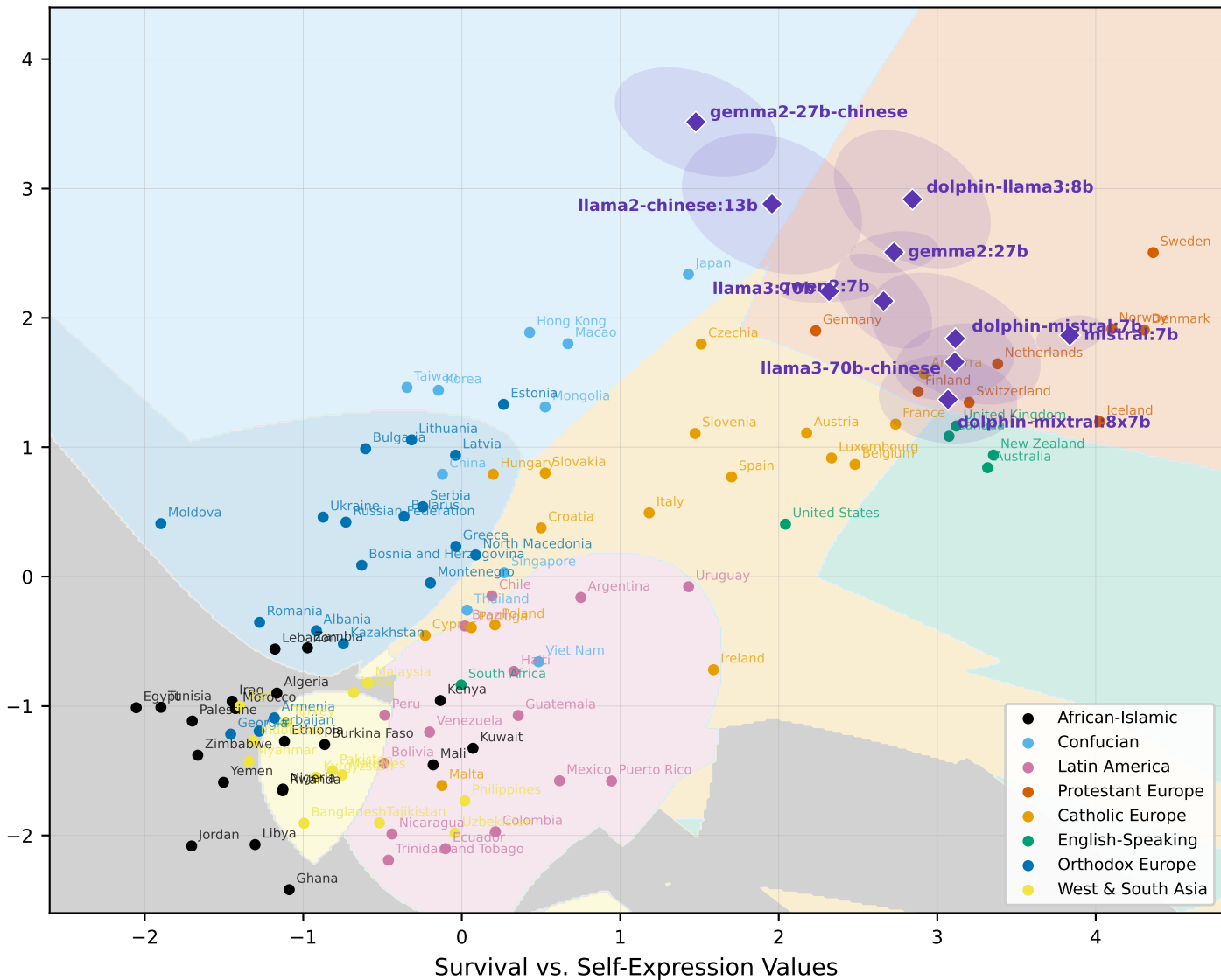
SVM cultural-region decision boundaries with LLM positions
